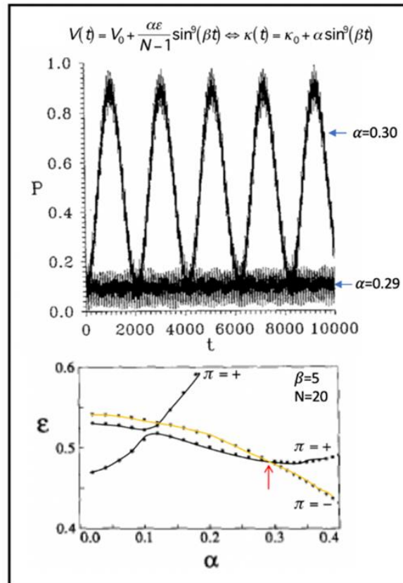
Fig.5 Upper part: Quantum tunneling probability for the initial state, corresponding to the symmetric combination of the pair of first excited nearly degenerate eigenstates of opposite parities which are obtained by diagonalization of the SU(2) Hamiltonian. In this example, N=20 fermions are in the presence of external driving with a frequency \beta=5 for two amplitudes \alpha=0.29 and \alpha=0.30 . Lower part: Selected Floquet quasienergies of different parity. For \alpha=0.29 , the positive parity quasienergy state (black line) crosses the negative parity (yellow line) member of the same doublet and leads to a halt in tunneling of the dominant component in the wave function [From Nucl. Phys. A 579, 144 (1994)]
