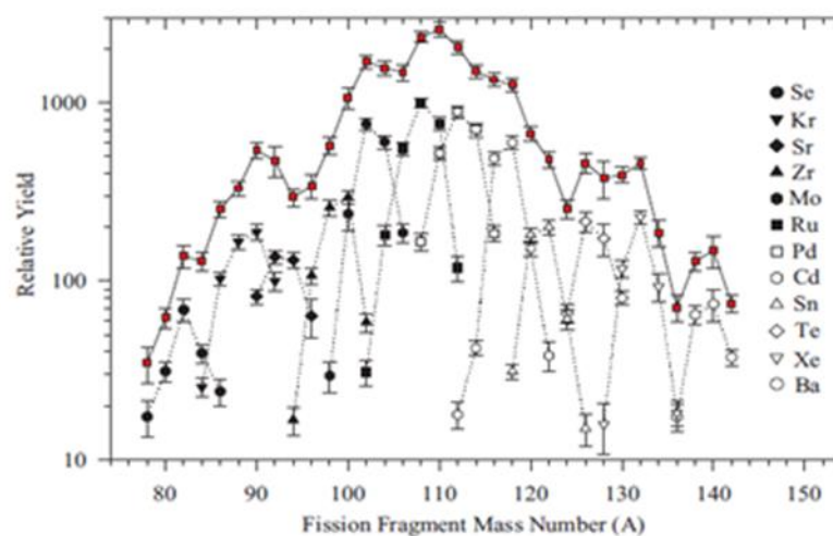
Fig.5 Relative fission fragment isotopic distribution from the reaction ^{208}\text{Pb}(^{18}\text{O},f) at E=90 MeV. Each complementary pair is represented by the same symbol with the light fragment shown by a filled symbol and the heavy fragment an open symbol [1].
