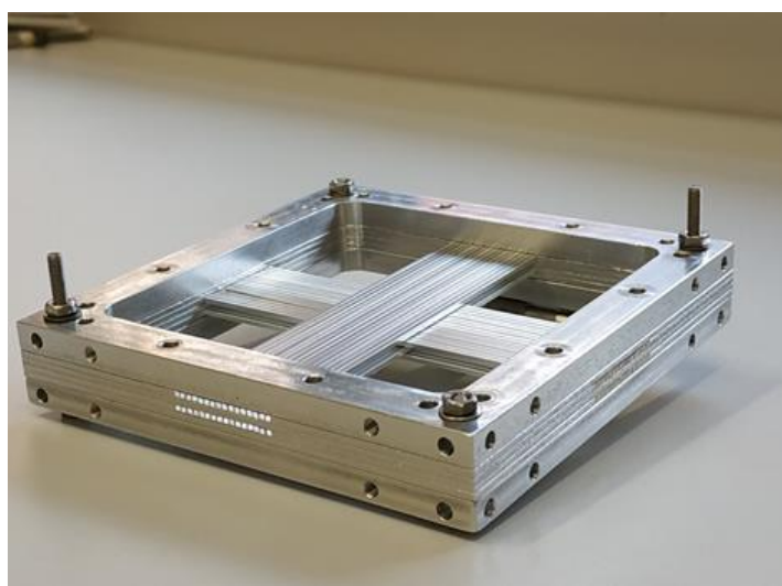
Fig.3 Photograph of a small-scale prototype of a SiFi-CC module.
