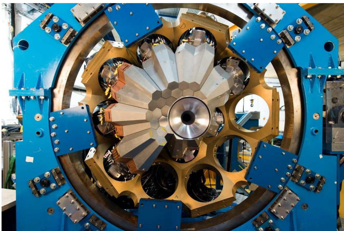
Fig.1 Part of the AGATA array (corresponding to approximately 1\pi of solid angle) installed at GANIL, France. Photo by P. Stroppa (CEA), https://www.ganil-spiral2.eu/press/
