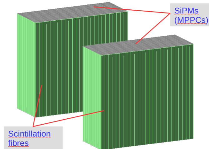
Fig.2 A sketch of the SiFi-CC setup: layers of scintillating fibers read out from both ends by silicon photomultipliers, stacked into two modules forming a Compton camera.
