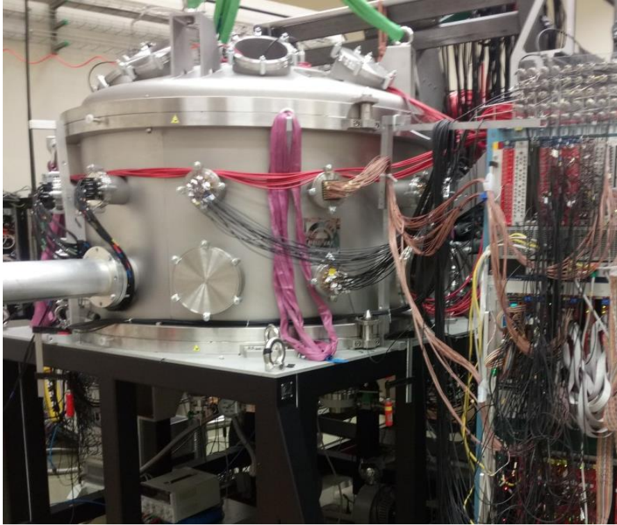
Fig.7 Photo of the large vacuum reaction chamber.
