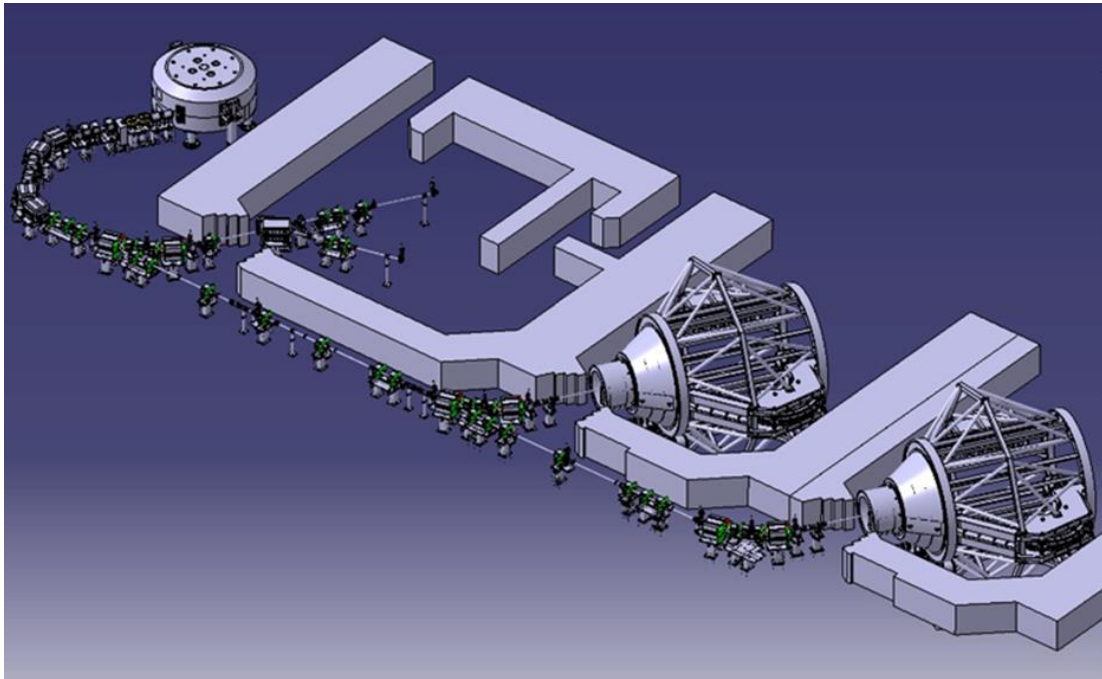
Fig.6 Schematic outline of the beamlines at the Cyclotron Centre Bronowice. The proton beam from the C-235 cyclotron is formed at the energy selector and transported to the experimental hall, eye treatment room and two scanning gantries.
