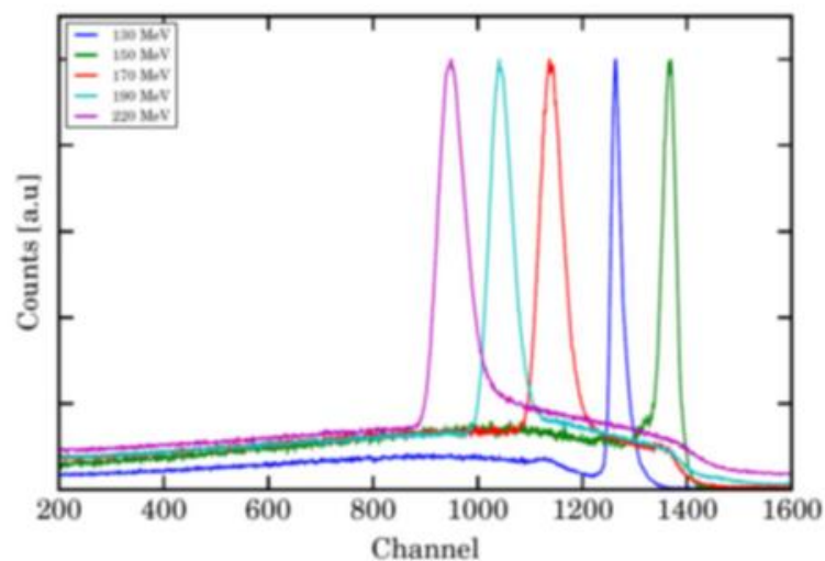
Fig.7 Spectra of protons for a 2"x2"x2" LaBr 3 from the PARIS detector for different energies (130-220 MeV). The spectra are normalized to have the same height of the proton peak.
