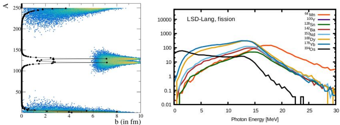
Fig.1 (Left) The distribution of nuclei after pre-equilibrium emission for the reaction \text{Xe}+\text{Sn}\rightarrow\text{Rf} at 12 A MeV. (Right) The Giant Dipole Resonances obtained by de-excitation of various nuclei in the fission channel.
