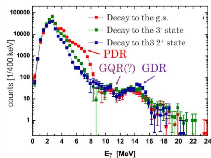
Fig.4 \gamma energy spectra corresponding to the decay of the excitation of various states in ^{208}\text{Pb}
