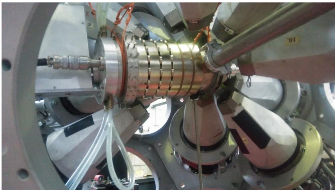
Fig.3 The electron spectrometer ULESE mounted inside the EAGLE Ge detector array at HIL UW
