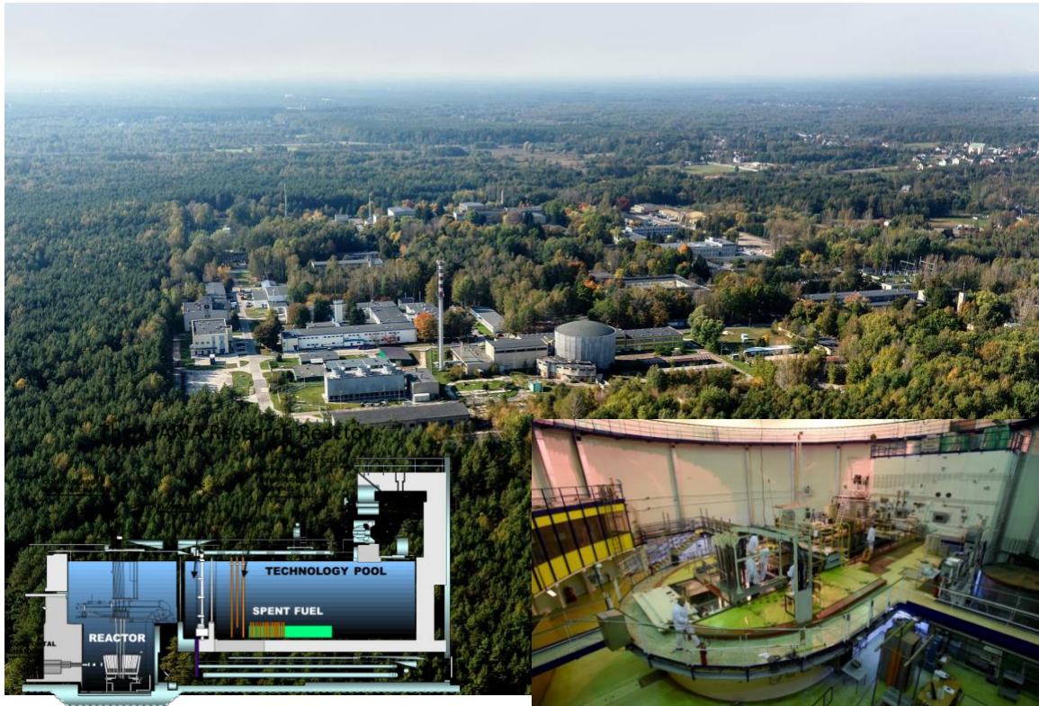
Fig.13 Technological overview of the MARIA reactor
