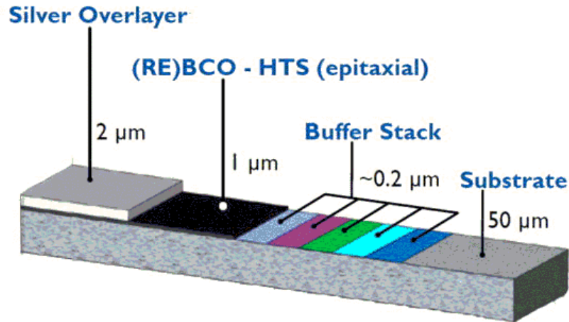
Fig.4 Illustrative drawing of the (RE)BCO tape structure [8].
