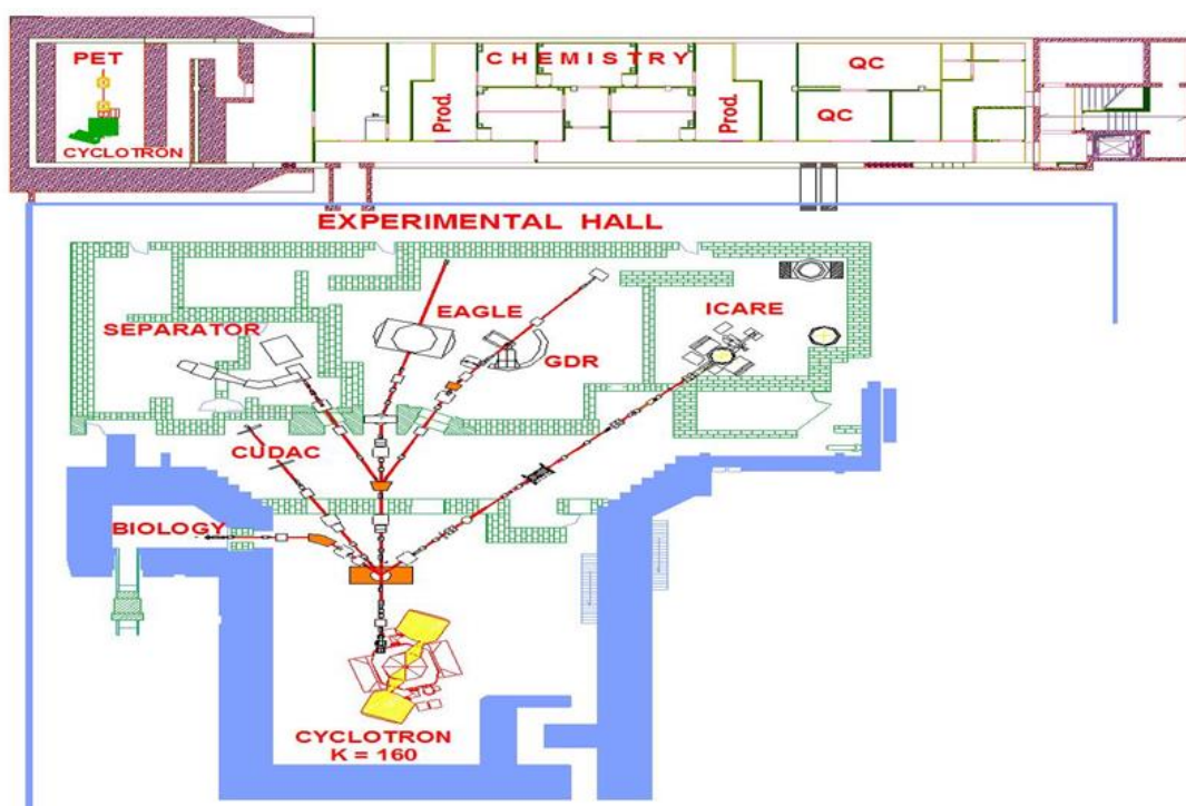
Fig.1 Layout of the HIL facility.
