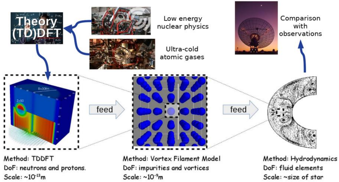
Fig.4 Scheme of the hierarchy of approaches to model the interior of a neutron star. First, microscopic information about the vortex properties, the vortex-nucleus interaction and impurity properties can be extracted from the TDDFT method based on quantified energy density functionals. Next, the vortex filament model is adjusted to these results and is used to extract dynamical vortex properties as it moves through the lattice of impurities (nuclear defects). Averaged results for volumes containing a large number of impurities constitute input for hydrodynamics, the results of which can finally be compared with observations.
