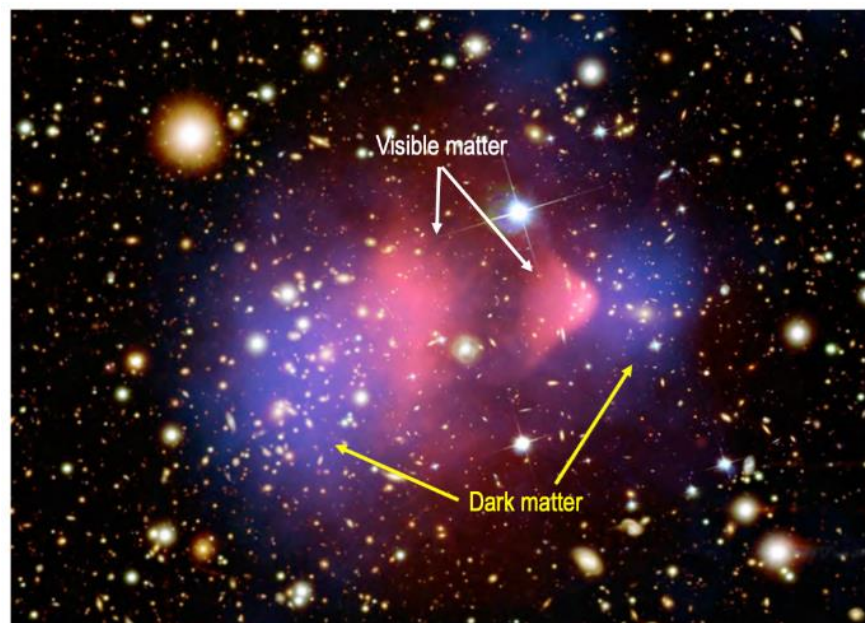
Fig. 7 The Bullet cluster (1E 0657-558): this picture of the collision of two clusters of galaxies, obtained by gravitational lensing, shows a separation between visible and dark matter.
