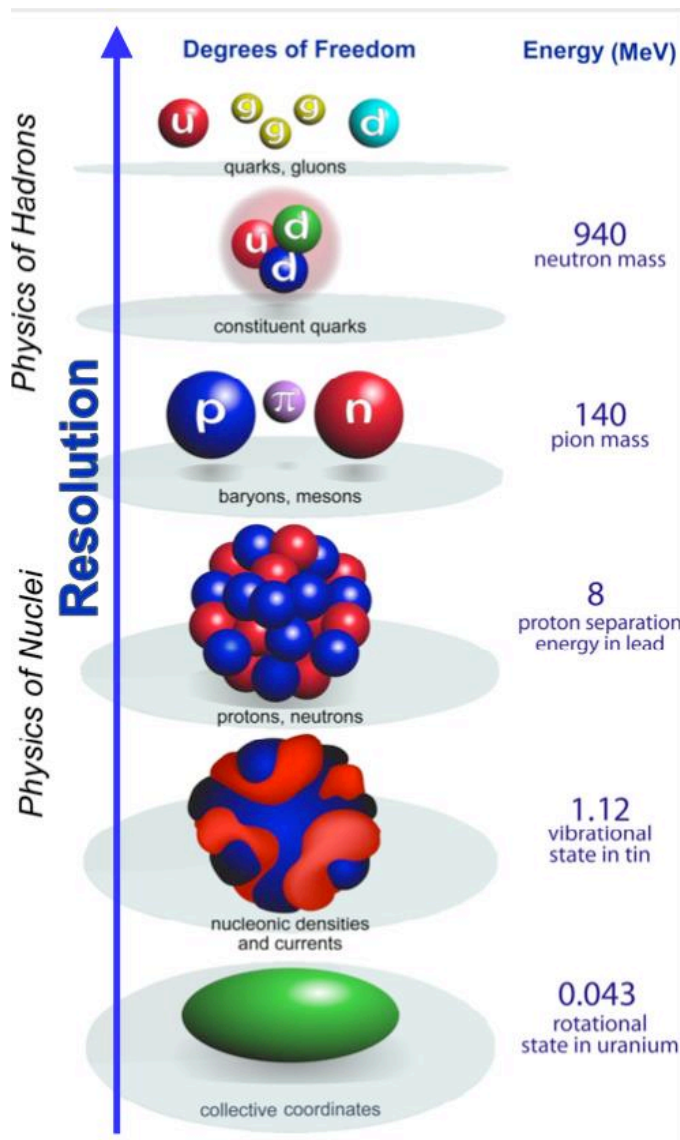
Fig.1 Nuclear degrees of freedom [Courtesy of W. Nazarewicz]
