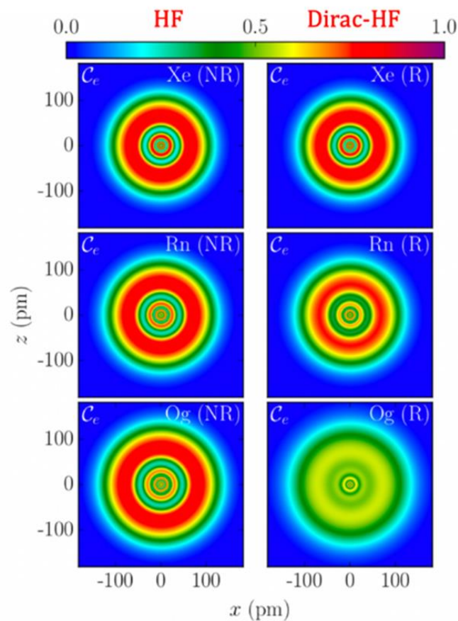
Fig.6 Electronic localization functions from nonrelativistic (NR, left) and Dirac-Hartree-Fock calculations (R, right) for the heavy noble gas atoms Xe (top), Rn (middle), and Og (bottom) [Phys. Rev. Lett. 120 , 053001 (2018)].
