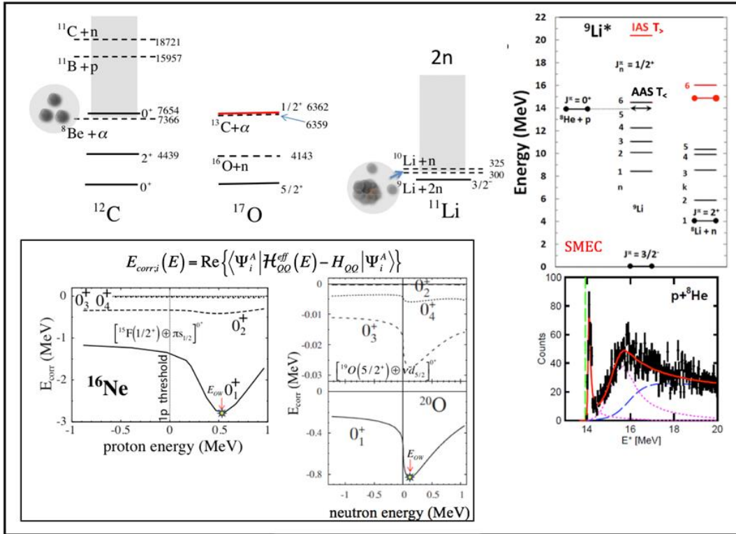
Fig.2 Various examples illustrating the emergence of nuclear clustering in the vicinity of the particle decay threshold. These include: the 0^+_2 Hoyle state in ^{12}\text{C} ; the narrow near-threshold 1/2^+_1 resonance in ^{17}\text{O} ; the halo ground state in ^{11}\text{Li} ; and the collective splinter of the anti-analog resonance in ^9\text{Li} . The insert of this figure shows the continuum-coupling correlation energy as a function of the particle energy in the vicinity of the proton decay channel in ^{16}\text{Ne} and the neutron decay channel in ^{20}\text{O} . The origin of the energy scale is at the threshold. The arrow points to the centroid of the energy opportunity window to form the aligned eigenstate which carries an imprint of the nearby decay channel. [Adapted from Prog. Theor. Phys. Supplement 196 , 230 (2012) Physics, 120; Acta Phys. Pol. B 45 , 331 (2014); Phys. Rev. C 97 , 044303 (2018)]
