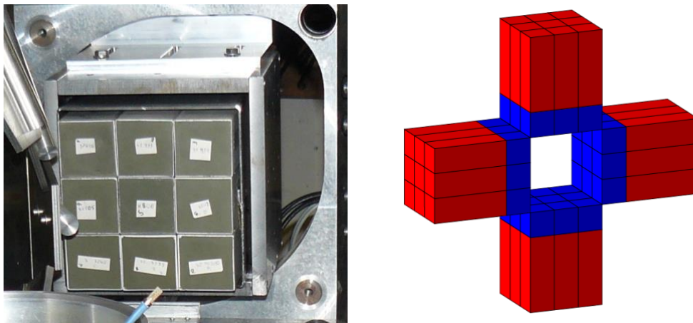
Fig.2 Left: PARIS, 9 phoswiches in cluster configuration - photo taken during preparation of an experiment at GANIL, Caen, France. Right: Schematic view of the possible arrangement of 4 PARIS clusters.
