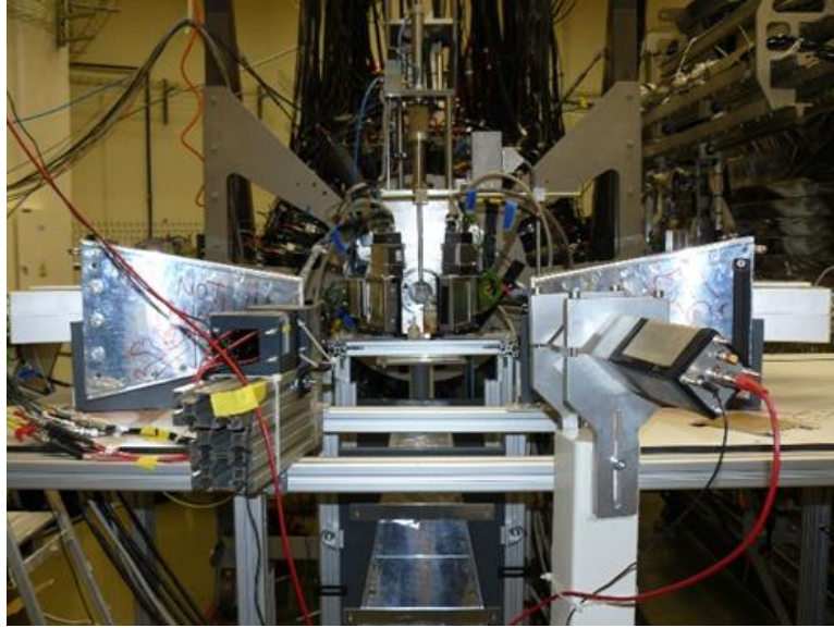
Fig.6 CALIFA petals in the experimental hall at CCB
