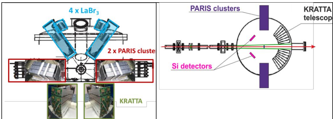
Fig.8 Schematic layout of the setup: left – view from the front; right – view from the top.
