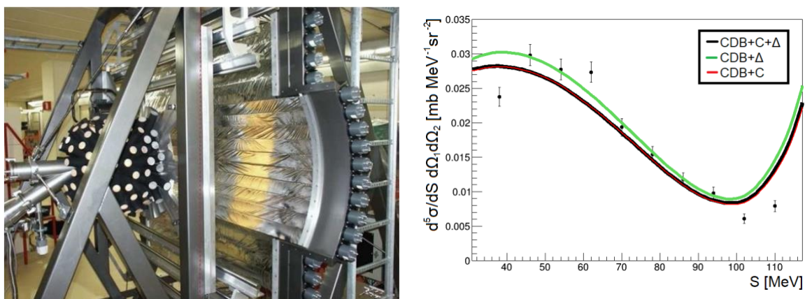
Fig.3 (Left) Photo of the BINA system. (Right) Preliminary differential cross section for one configuration ( \theta_1=16^\circ , \theta_2=28^\circ , \varphi_{12}=160^\circ ) of the dp breakup reaction at 108 MeV (theoretical calculations by A. Deltuva).
