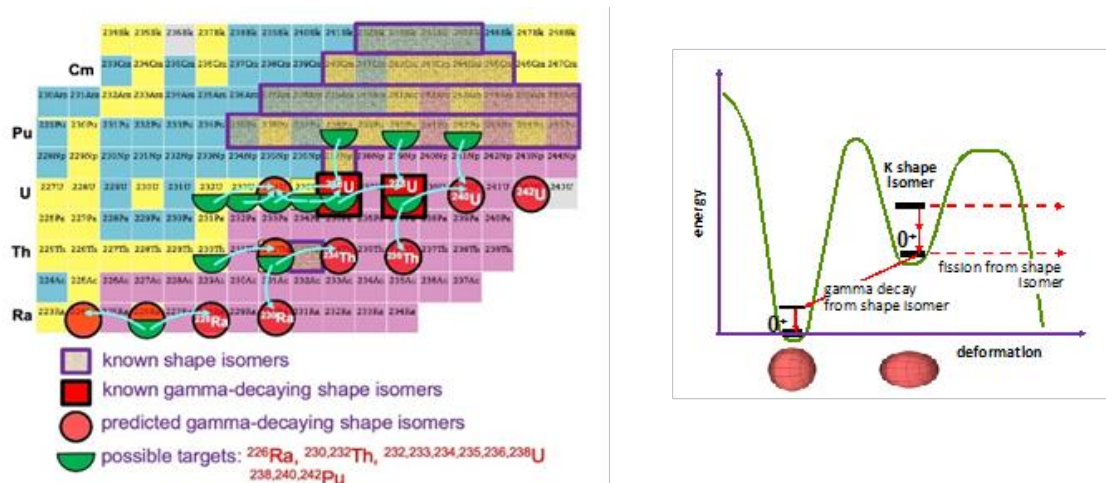
Fig.1 Map (left) of actinide nuclei in which \gamma -decaying shape isomers were identified (solid red squares) or predicted (solid red circles) are shown. Possible targets for studies using one- or two-nucleon sub-barrier transfer reactions induced by very heavy beams are displayed as half circles. The right-hand side shows a schematic illustration of a K-shape-isomer decay
