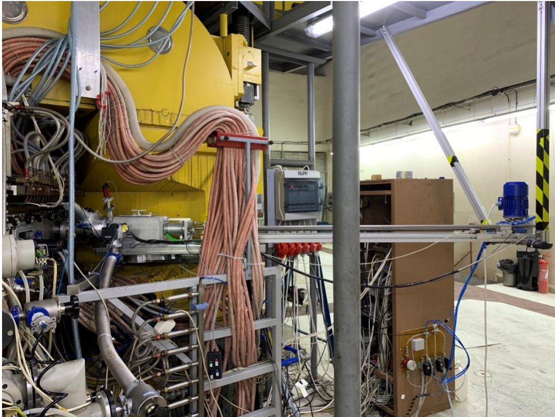
Fig.10 A view of the target station for the U-200P cyclotron.
