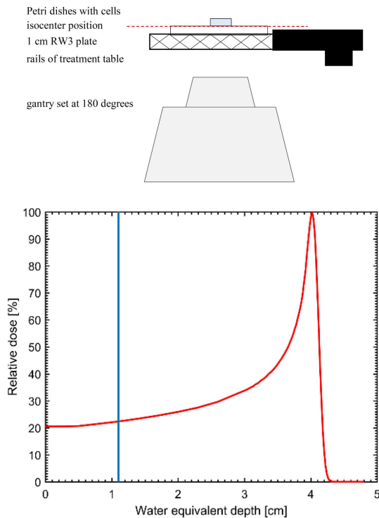
Fig. 1. The irradiation setup (top). The exemplary depth dose distribution of 70 MeV proton beam in water. The blue line marks the position of the cell at 1.1 cm water equivalent depth (bottom).
