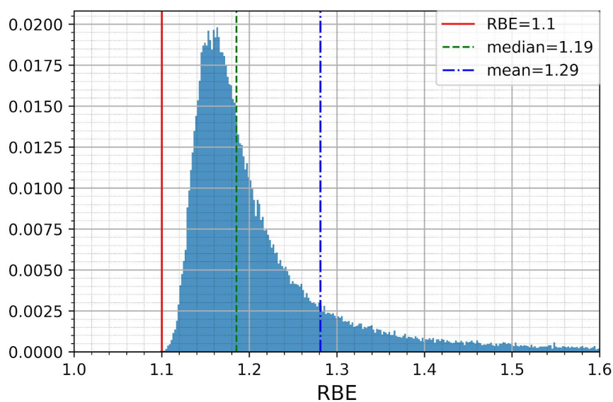
Fig 6. Histogram drawn from the distribution of RBE values for protons of energy 16.7 MeV, dose 2.0 Gy and biological endpoint characterized by \alpha/\beta = 2.0 Gy in the LQ model.
