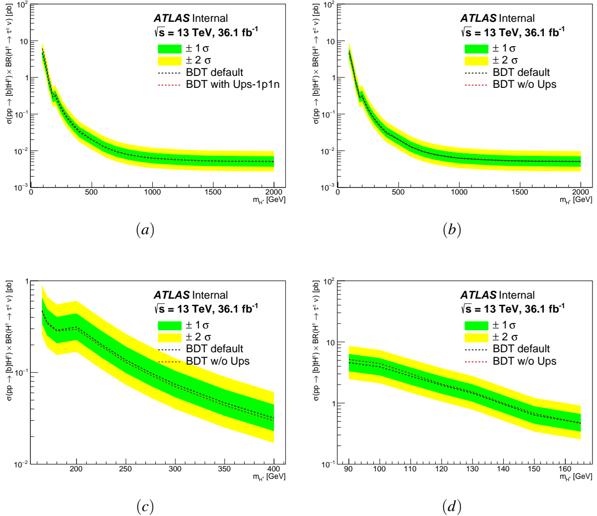
Figure 5.20: Juxtaposition of expected 95% CL exclusion limits on \sigma(pp \rightarrow [b]tH^\pm) \times \text{BR}(H^\pm \rightarrow \tau^\pm \nu) for charged Higgs boson production as a function of m_{H^\pm} in 36.1 \text{ fb}^{-1} of pp collision data at \sqrt{s} = 13 \text{ TeV} for two cases: (a) default BDT output and an alternative BDT where \Upsilon for H^\pm masses in the range 90 – 400 GeV is used as an input variable in the final BDT discriminant for events where \tau_{\text{had-vis}} decays only on one charged and one neutral meson (BDT with Ups-1p1n); (b)-(d) default BDT output and an alternative BDT where p_T^{\tau\text{-track}} in place of using \Upsilon for H^\pm masses in the range 90 – 400 GeV is used as an input variable in the final BDT discriminant for events where \tau_{\text{had-vis}} has only one associated track (BDT w/o Ups).
