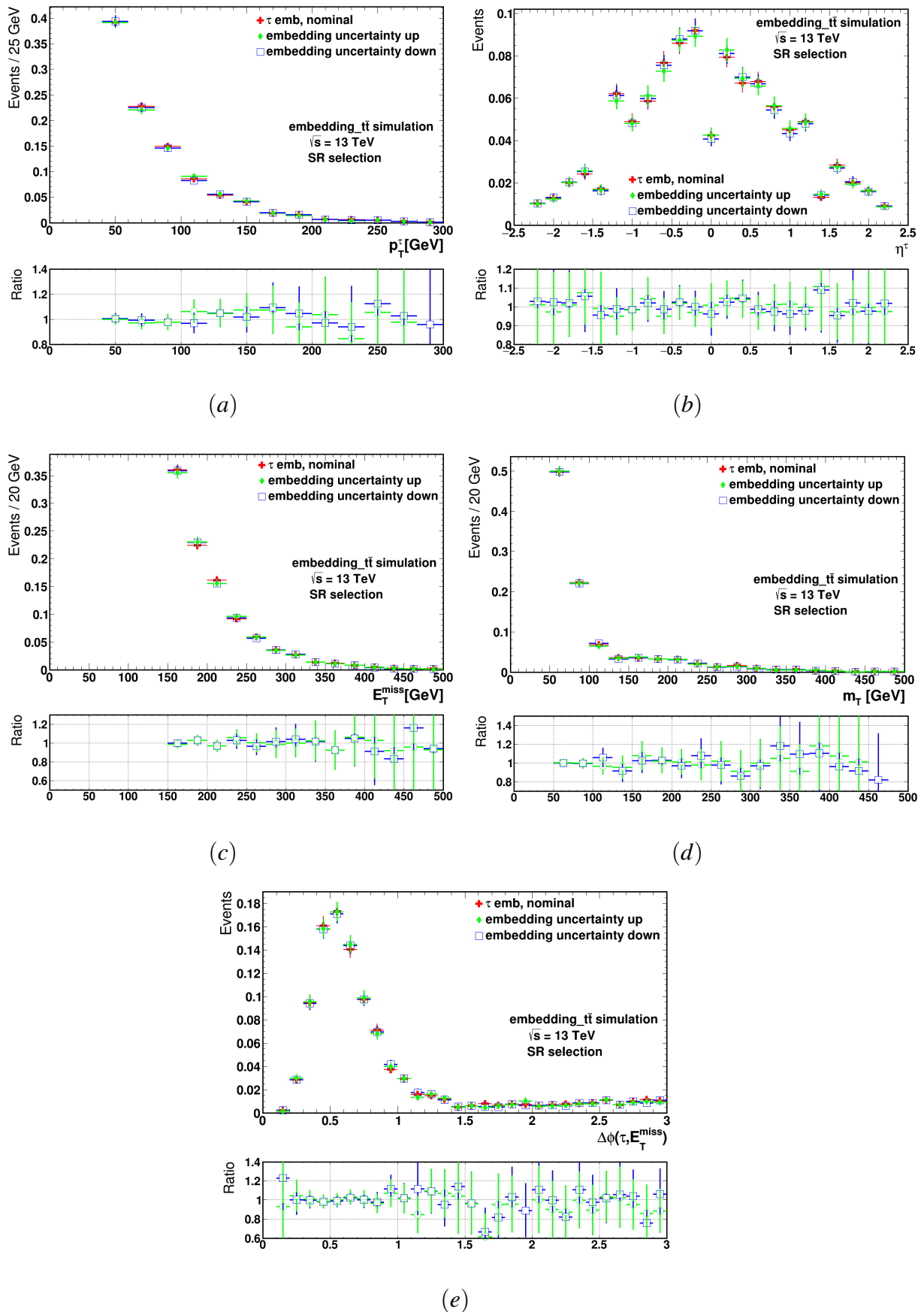
Figure 6.15: Effect of the embedding uncertainties on the shape of (a) p_T , (c) E_T^{\text{miss}} , (b) \eta , (d) m_T and (e) \Delta\phi distributions after applying the SR selection for embedded t\bar{t} MC simulation.
