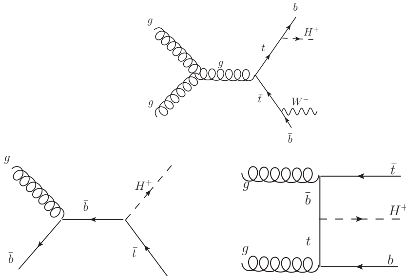
Figure 2.3: Leading Feynman diagrams for the charged Higgs boson production processes in the proton-proton collision: top quark decay (upper) and associated top production in five-flavour (5FS- bottom left) and four-flavour (4FS- bottom right) scheme.
