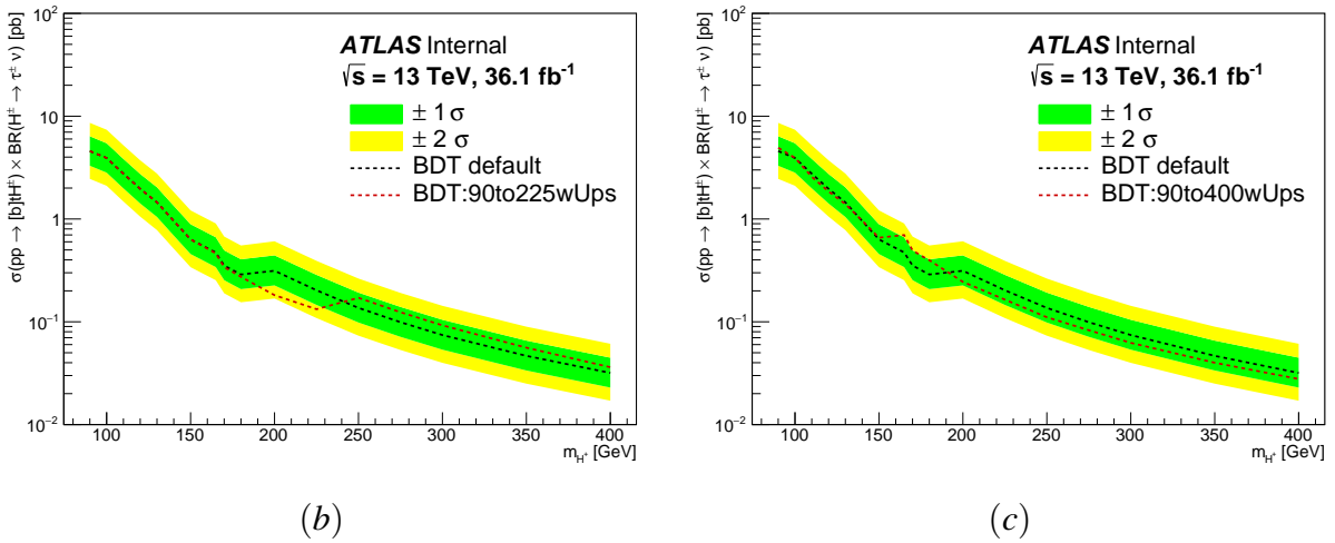
Figure 5.19: Juxtaposition of expected 95% CL exclusion limits on \sigma(pp \rightarrow [b]tH^\pm) \times \text{BR}(H^\pm \rightarrow \tau^\pm \nu) for two cases: (a) default BDT output and an alternative BDT where in place of using \Upsilon in training for H^\pm masses in the range 90-400 GeV it is used for H^\pm masses in the range 90-225 GeV for events where \tau_{\text{had-vis}} has only one associated track; (b) default BDT output and an alternative BDT where \Upsilon is used in the training for events where \tau_{\text{had-vis}} has only one associated track, for H^\pm masses in the range 90-400 GeV divided into two mass bins: 90-120 and 130-400 GeV.
