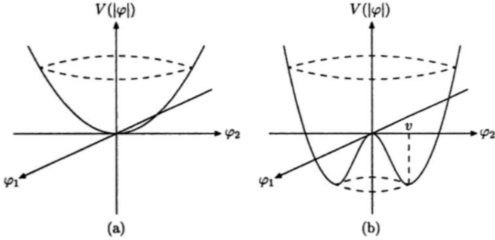
Figure 2.1: The potential for the \varphi field in the basis of two real degrees of freedom \varphi_1 and \varphi_2 . Two cases are shown: without (a) and with (b) spontaneous symmetry breaking. From [16].
