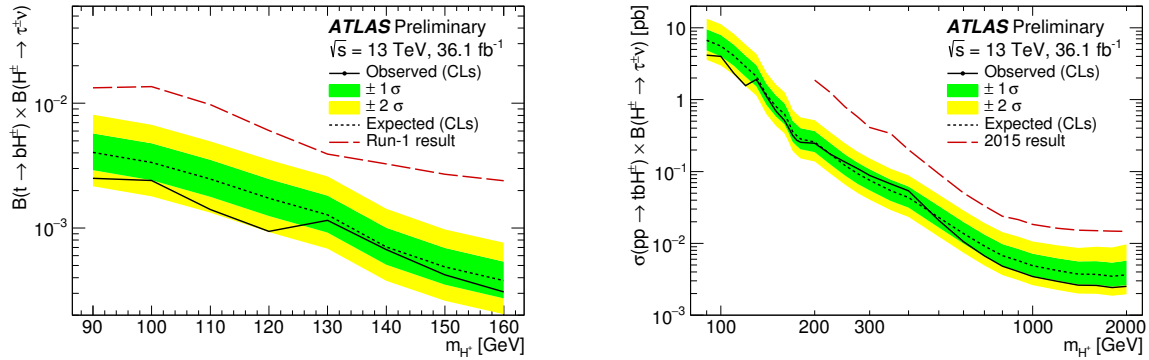
Figure 7.2: Observed and expected 95% CL exclusion limits on (right) \sigma(pp \rightarrow [b]tH^\pm) \times B(H^\pm \rightarrow \tau^\pm \nu) and (left) B(t \rightarrow bH^\pm) \times B(H^\pm \rightarrow \tau^\pm \nu) as a function of the charged Higgs boson mass in 36.1 \text{ fb}^{-1} of pp collision data at \sqrt{s} = 13 \text{ TeV} , after combination of the \tau_{\text{had-vis}}+\text{jets} and \tau_{\text{had-vis}}+\text{lepton} final states. In the case of the expected limits, one- and two-standard-deviation uncertainty bands are also shown. In the H^\pm mass range of 90–160 GeV, the limits obtained with the Run-1 data [39] are also shown. From [12].
