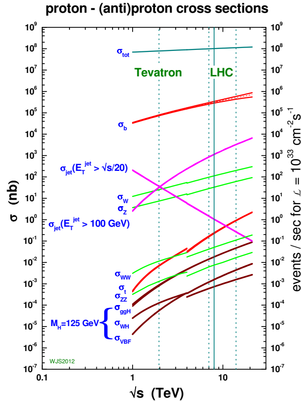
Figure 3.8: Cross sections for \sqrt{s} in range 0.1-20 TeV [57].
