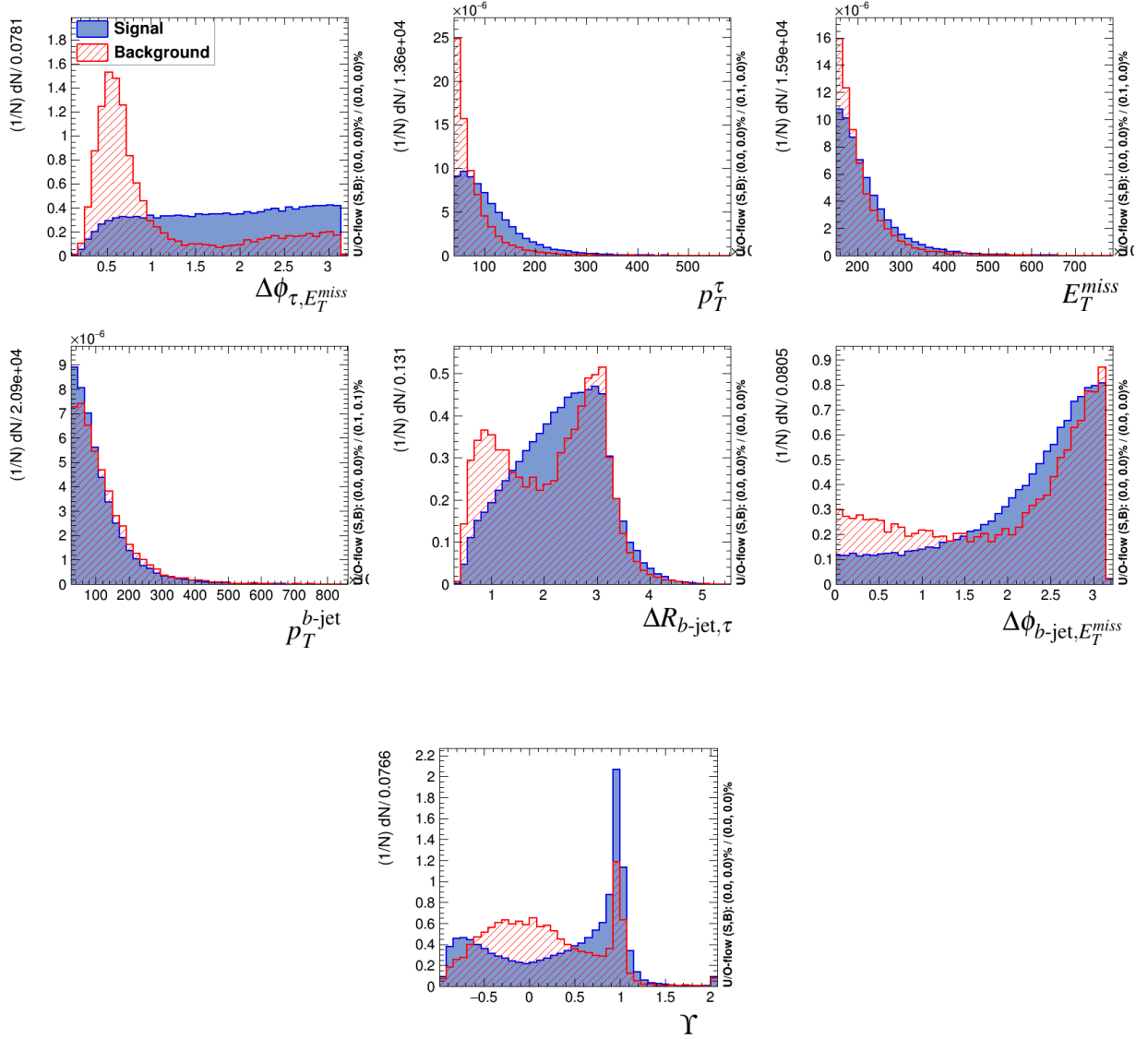
Figure 5.8: Distributions of input variables for BDT-training within 200-400 GeV mass bin. Signal is presented as a blue, solid histogram; top background (as estimated from MC) is presented as a red, dashed histogram. Histograms are arbitrarily normalised.
