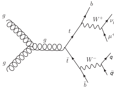
Figure 6.3: Feynman diagram of the Standard Model process of top quark pair production with W^\pm \rightarrow \mu^\pm \nu decay used for the embedding.
