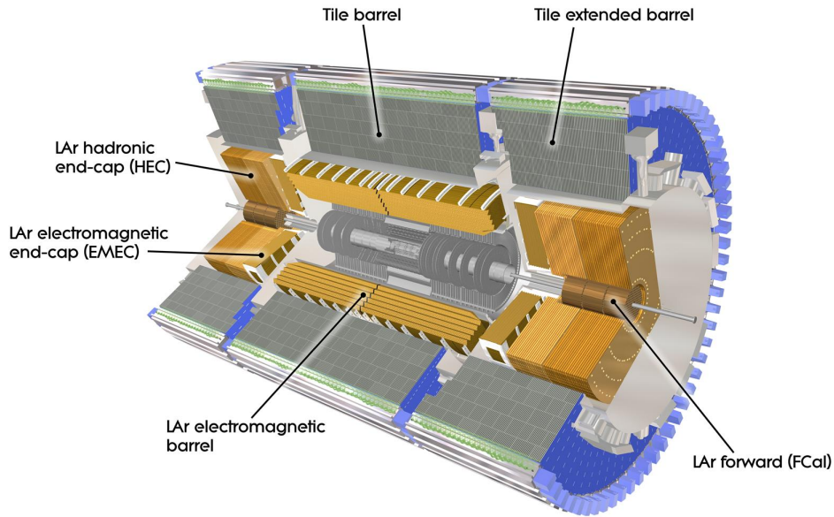
Figure 3.4: Cut-away view of the ATLAS calorimetry. The three distinct cylinders, barrel and end-caps, are visible. The smaller radial regions use the LAr technology requiring cryostats, whereas the outer cylinders use scintillator tiles embedded in an iron absorber structure. The end-caps can be moved longitudinally along the LHC beam line for creating access space to maintain the barrel region [2].
