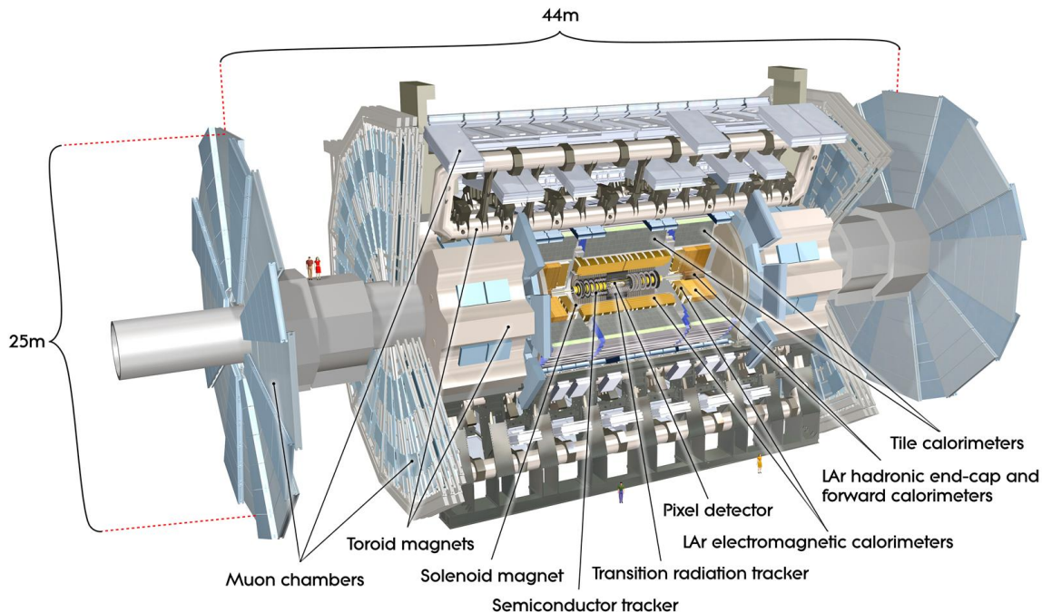
Figure 3.2: Schematic cut-away view of the ATLAS detector showing the different layers of the inner detector, the calorimeters, toroid magnets and muon spectrometer [2].
