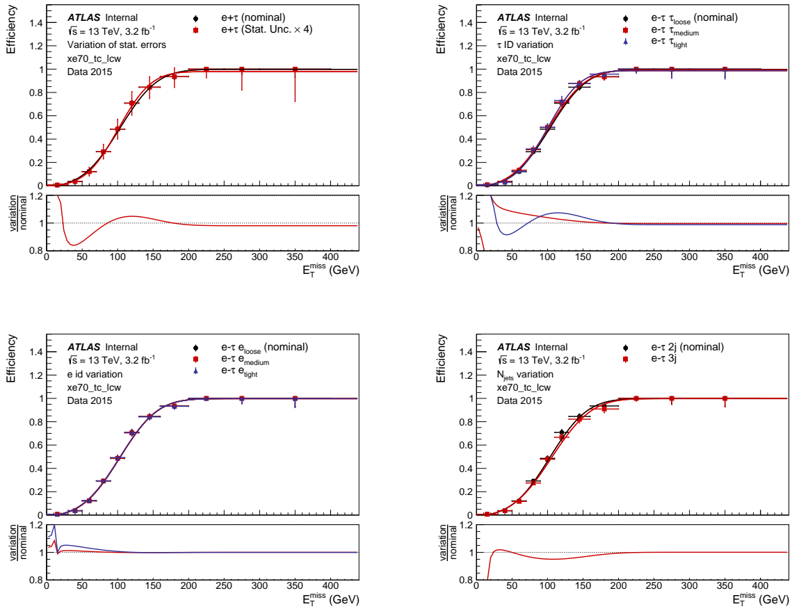
Figure 6.12: Trigger efficiencies in data and corresponding fits for the e+\tau_{\text{had-vis}} selection and HLT_xe70_tc_lcw trigger (a) where the errors on the fitted points have been increased to 4\times Stat. error. (b) when varying the \tau_{\text{had-vis}} identification between loose (nominal), medium and tight ; (c) when varying the e identification between loose (nominal), medium and tight ; (d) when increasing the requirement on the number of jets to \geq 3 . The ratio plots show the fit of the variation divided by the fit of the nominal case. From [33].
