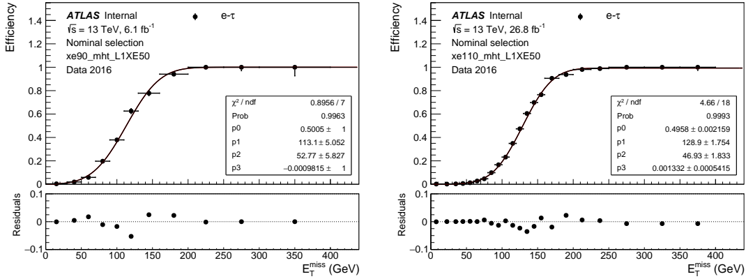
Figure 4.5: Trigger efficiency and corresponding fit with the \tau_{\text{had-vis}} selection for HLT_xe90_mht_L1XE50 (top left) and HLT_xe110_mht_L1XE50 (top right) triggers. From [33].
