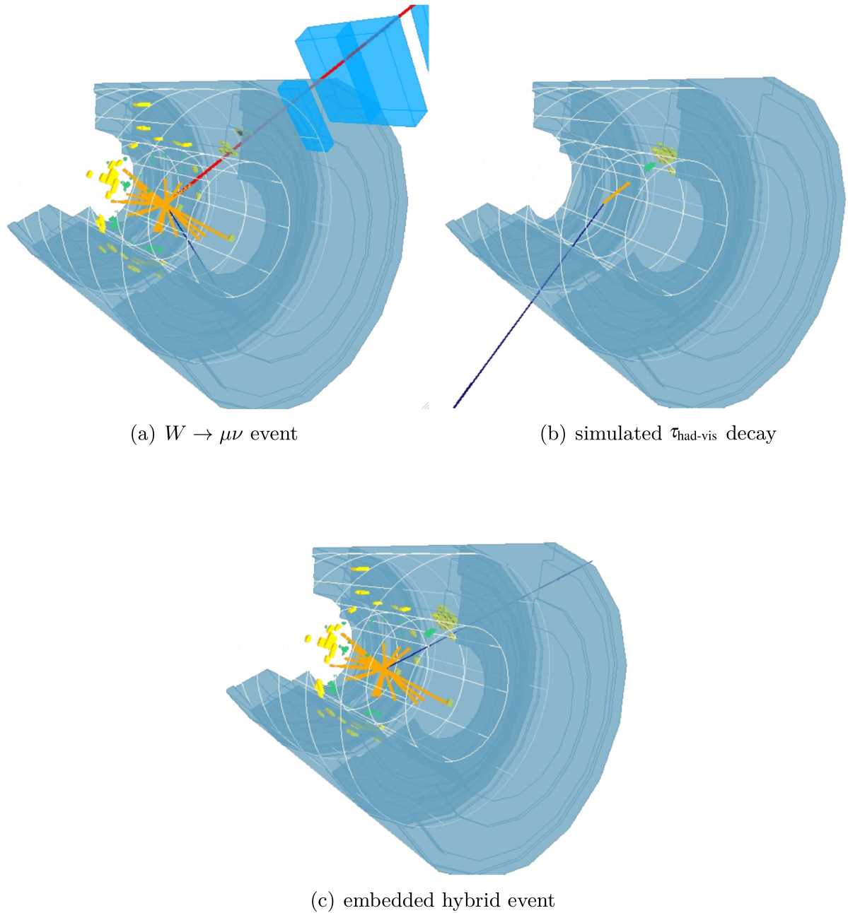
Figure 6.5: ATLAS Event Display showing (a) W^\pm \rightarrow \mu^\pm \nu event, (b) simulated hadronic \tau lepton decay and (c) the embedded hybrid event in a cut-away view of the ATLAS detector. The muon is shown in red and traverses the muon chambers, E_T^{miss} is shown in dark blue. The \tau_{\text{had-vis}} candidate can be identified by its track (orange) and deposits in the calorimeters (green and yellow). From [137].
