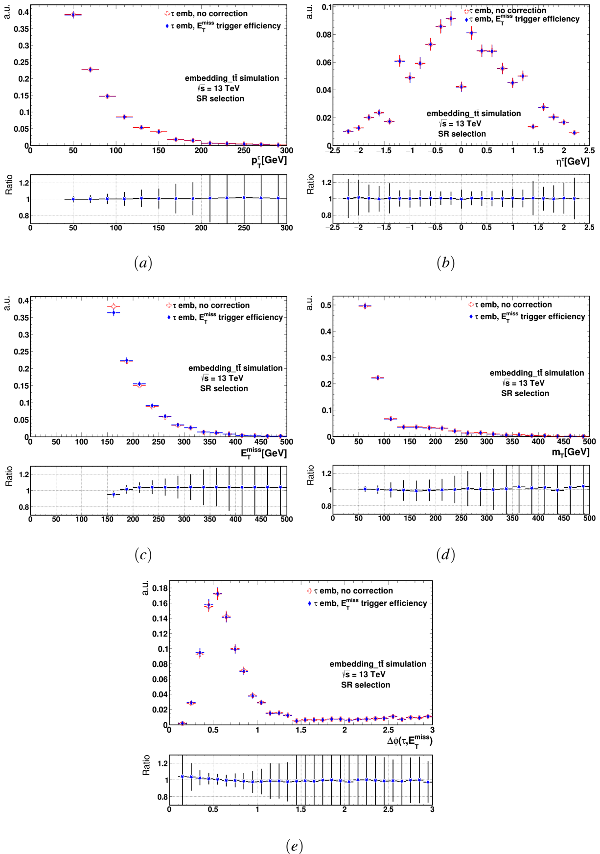
Figure 6.9: Juxtaposition of (a) p_T^\tau , (b) \eta^\tau , (c) E_T^{miss} , (d) m_T and (e) \Delta\phi(\tau, E_T^{miss}) distributions before and after applying the correction on E_T^{miss} trigger efficiency for embedded t\bar{t} MC simulation.
