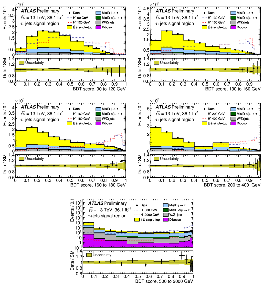
Figure 7.1: BDT score distributions in the five mass ranges used for the BDT trainings, after a fit to the data with the background-only hypothesis. The uncertainty bands in the ratio plots include both the statistical and systematic uncertainties. The normalisation of the signal (shown for illustration) corresponds to the integral of the background. From [12].
