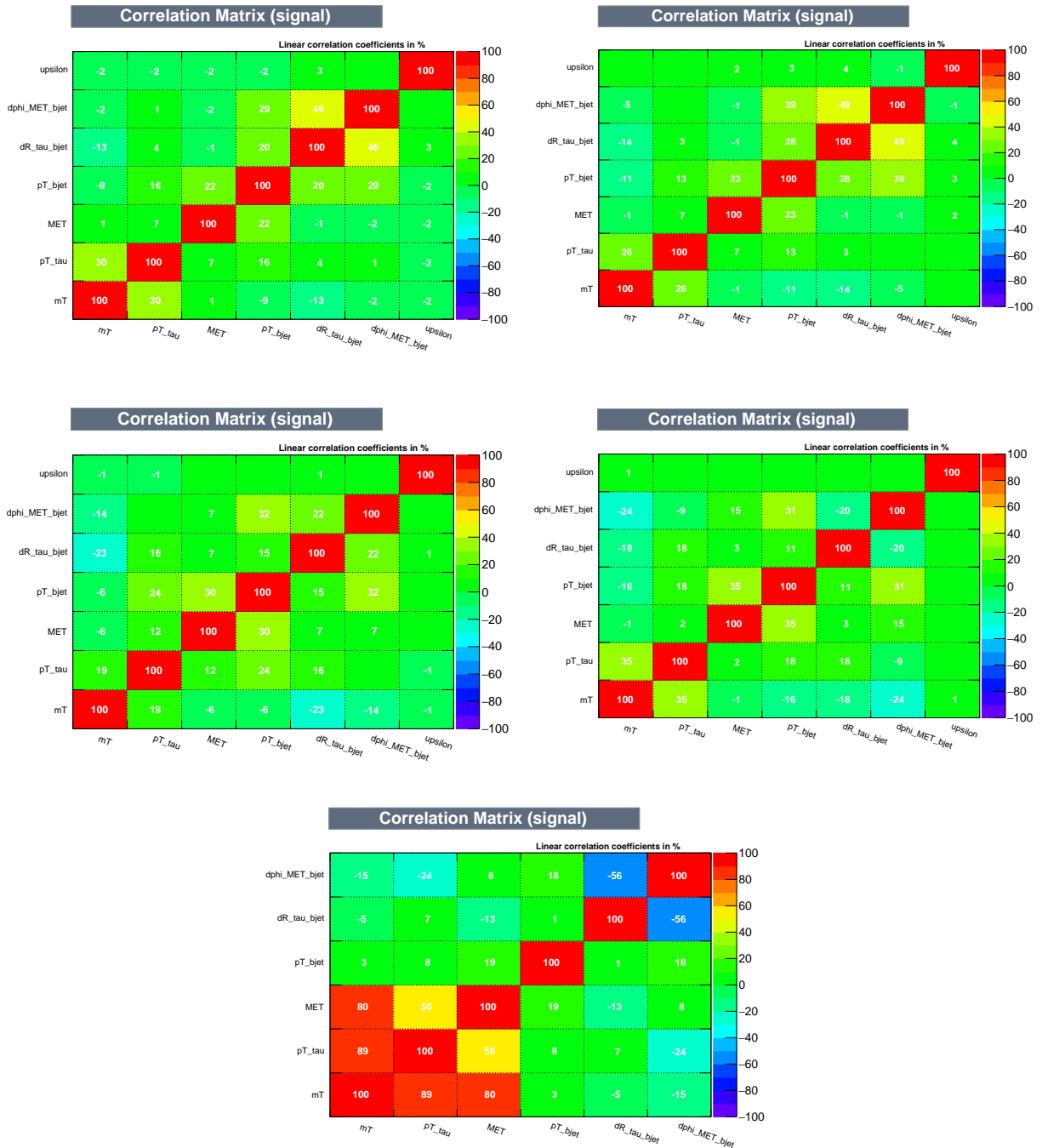
Figure 5.15: Correlation matrix of alternative BDT input variables, where m_T in place of \Delta\phi_{\tau,E_T^{\text{miss}}} is used (see Fig. 5.10 for comparison), for the signal. The five H^\pm mass ranges used in the BDT training are presented, 90–120 GeV (top left), 130–160 GeV (top right), 160–180 GeV (middle left), 200–400 GeV (middle right) and 500–2000 GeV (bottom). Where: \epsilon = \Upsilon ; d\phi_{b\text{-jet},E_T^{\text{miss}}} = \Delta\phi_{b\text{-jet},E_T^{\text{miss}}} ; dR_{b\text{-jet},\tau} = \Delta R_{b\text{-jet},\tau} ; p_T^{b\text{-jet}} = p_T^{b\text{-jet}} ; MET = E_T^{\text{miss}} ; p_T^{\tau} = p_T^{\tau} and m_T = m_T .
