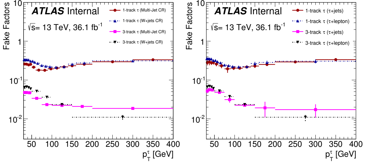
Figure 4.6: Fake factors parameterised as a function of p_T^\tau and the number of charged \tau decay products (two categories: 1-prong and 3-prong), as obtained in the multi-jet and W +jets CRs (left), as well as after reweighting by \alpha_{\text{MJ}} (right). The errors shown come from the statistical uncertainty in a given p_T^\tau bin (left) and with additional systematical uncertainties obtained from the combination in a given p_T^\tau bin (right). Note that this thesis describes searching H^\pm in \tau_{\text{had-vis}} +jets channel, whereas on the right plot also results for \tau_{\text{had-vis}} +lepton channel are shown. From [33].
