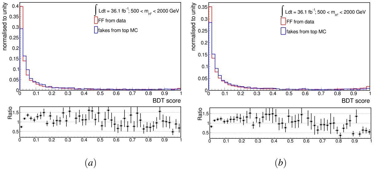
Figure 5.17: Juxtaposition of BDT score, for training in the mass range 500–2000 GeV, for events with the misidentified \tau_{\text{had-vis}} candidates as estimated with the FF method and as taken from the simulated top background samples for two training cases: (a) in the training the misidentified \tau_{\text{had-vis}} candidates estimated with the FF method are included, (b) in the training events the misidentified \tau_{\text{had-vis}} candidates are taken from the simulated top background samples are included.
