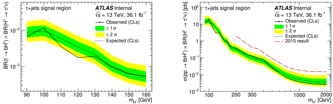
Figure 7.3: Observed and expected 95% CL exclusion limits on \text{BR}(t \rightarrow bH^\pm) \times \text{BR}(H^\pm \rightarrow \tau^\pm \nu) (left) and \sigma(pp \rightarrow [b]tH^\pm) \times \text{BR}(H^\pm \rightarrow \tau^\pm \nu) (right) for charged Higgs boson production as function of m_{H^\pm} in 36.1 \text{ fb}^{-1} of pp collision data at \sqrt{s} = 13 \text{ TeV} for the \tau_{\text{had-vis}}+\text{jets} channel. From [33].
