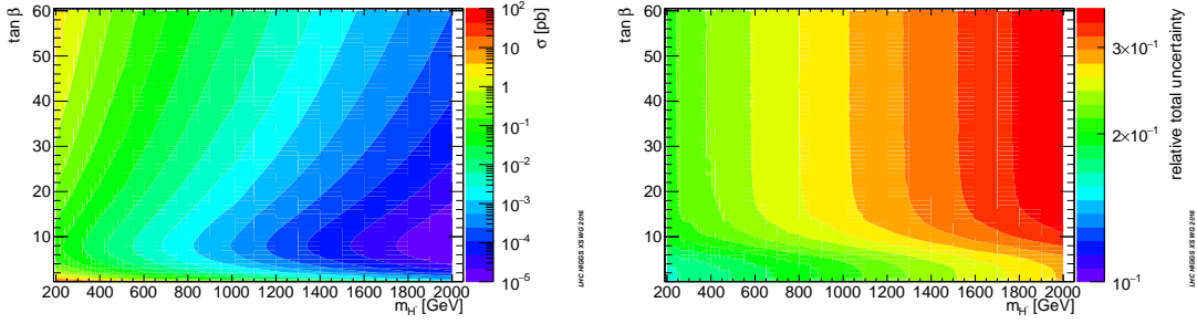
Figure 2.5: Two-dimensional plot of the charged Higgs boson production cross section (left) and average relative uncertainty (right) as a function of \tan\beta and m_{H^\pm} values in the 4FS of the 2DHM [33].
