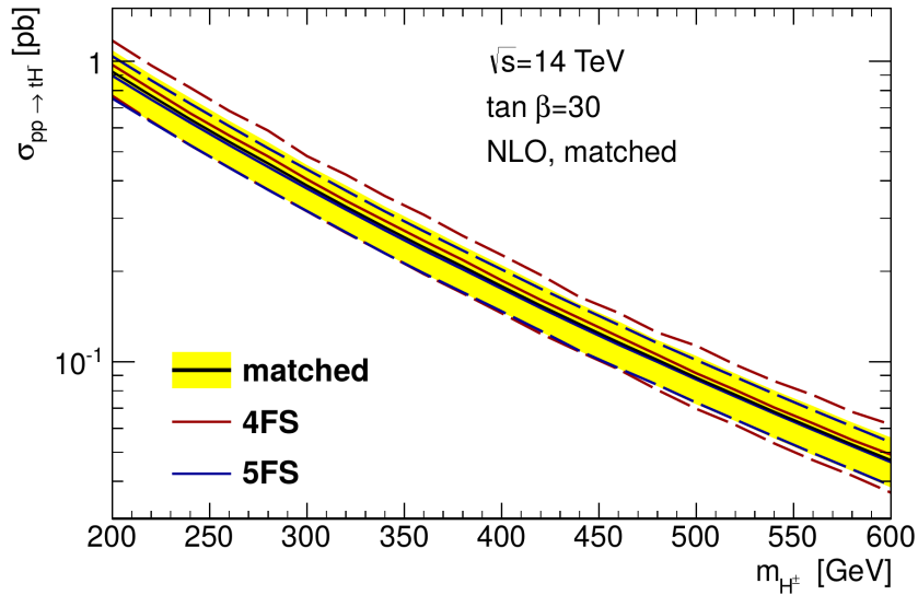
Figure 2.4: Production cross section for charged Higgs bosons as a function of m_{H^\pm} for \tan\beta = 30 at a center-of-mass energy of \sqrt{s} = 13 TeV. Values are shown for the 5FS, 4FS schemes and matched, where the red and blue dashed lines indicate the systematic uncertainties on the 4FS and 5FS, respectively, and the yellow band shows the uncertainty on the matched cross sections [31].
