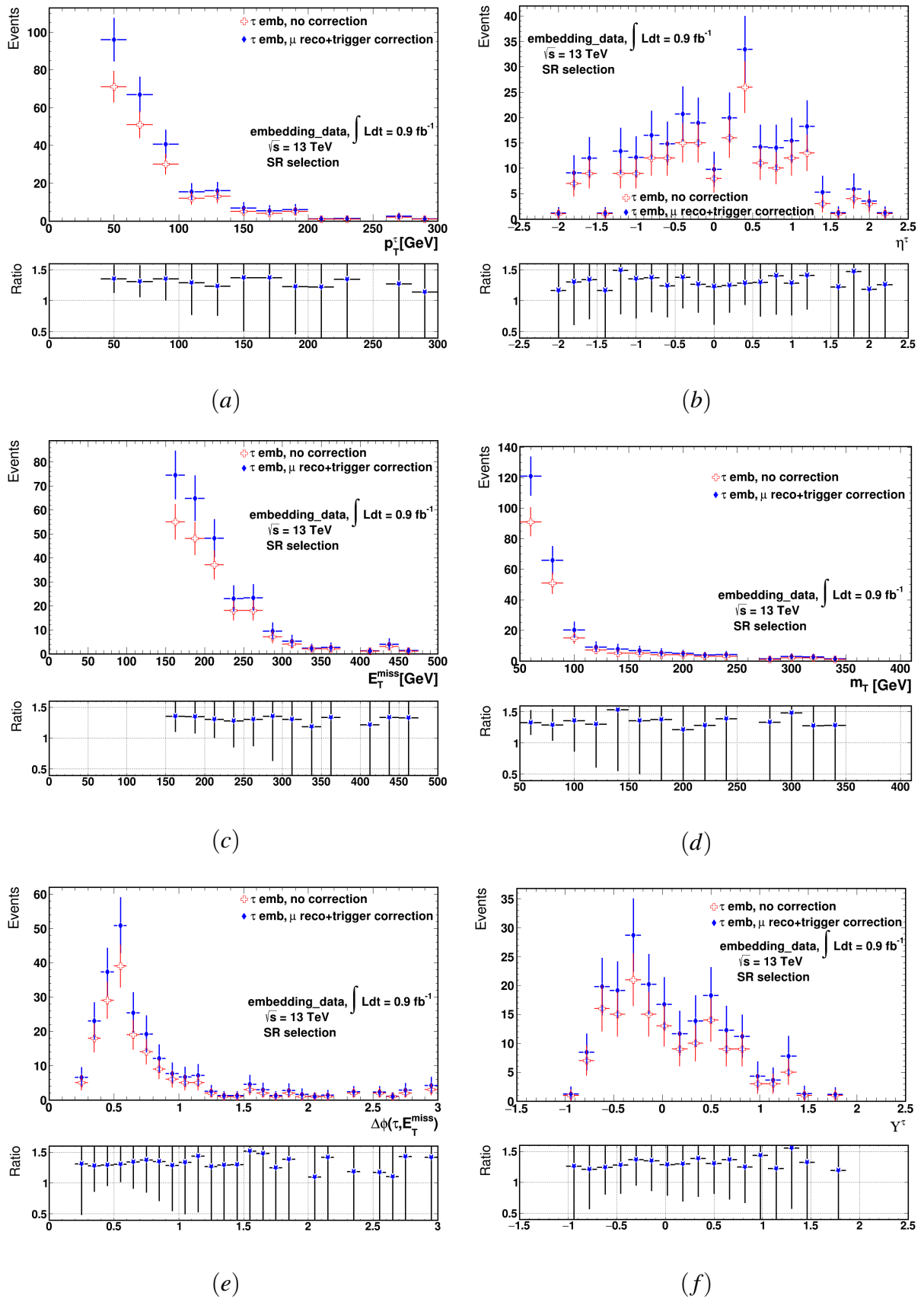
Figure 6.7: Juxtaposition of (a) the embedded \tau transverse momentum p_T^\tau and (b) pseudorapidity \eta^\tau , (c) E_T^{miss} , (d) m_T , (e) \Delta\phi(\tau, E_T^{miss}) and (f) Y^\tau observables before and after applying the correction factors on the \mu reconstruction and trigger efficiencies for the data embedding.
