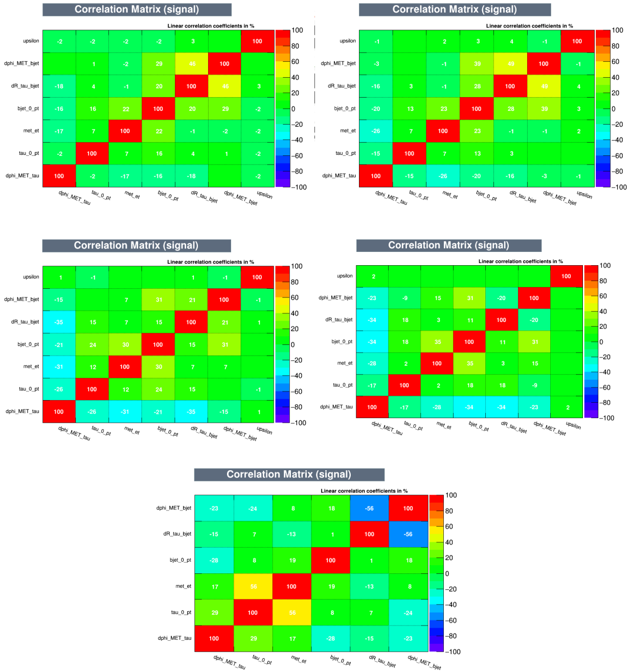
Figure 5.10: Correlation matrix of BDT input variables for the signal. The five H^\pm mass ranges used in the BDT training are presented, 90–120 GeV (top left), 130–160 GeV (top right), 160–180 GeV (middle left), 200–400 GeV (middle right) and 500–2000 GeV (bottom). Where: \text{upsilon} = \Upsilon ; d\phi_{MET,bjet} = \Delta\phi_{b\text{-jet}, E_T^{miss}} ; dR_{\tau,bjet} = \Delta R_{b\text{-jet}, \tau} ; bjet_{0,pt} = p_T^{b\text{-jet}} ; met_{et} = E_T^{miss} ; \tau_{0,pt} = p_T^\tau and d\phi_{MET,\tau} = \Delta\phi_{\tau, E_T^{miss}} .
