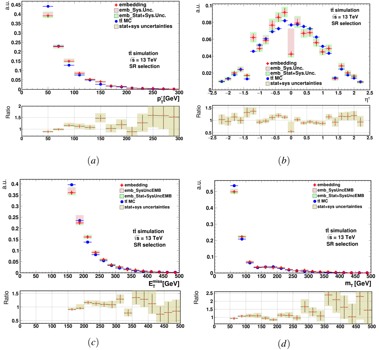
Figure 6.16: Juxtaposition of (a) p_T^\tau , (b) \eta^\tau , (c) E_T^{miss} and m_T of default and MC embedded t\bar{t} simulation after applying the SR selection with all corrections and systematic uncertainties related to the embedding procedure. The hatched red areas indicate the embedding-related systematic uncertainties, whereas the hatched green areas indicate the embedding-related statistical and systematic uncertainties.
