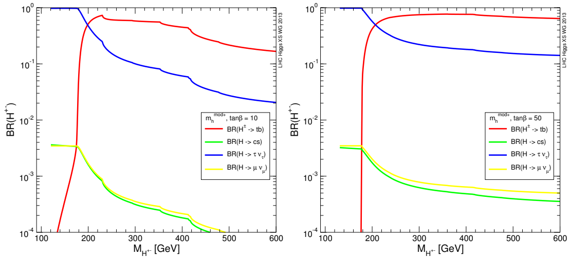
Figure 2.6: Branching fractions of the charged Higgs boson as a function of m_{H^\pm} , for \tan\beta values of 10 (left) and 50 (right), in the m_h^{\text{mod}+} scenario of the MSSM [33].
