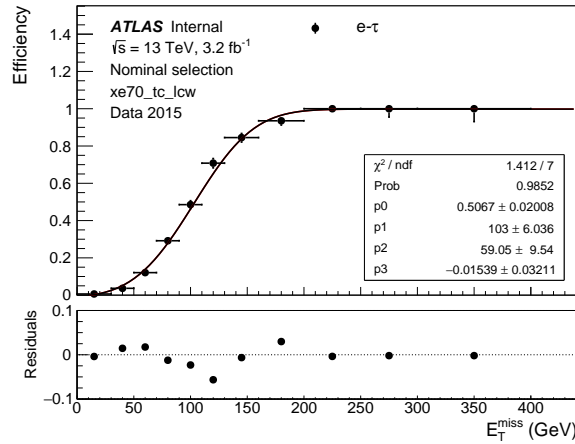
Figure 6.8: Trigger efficiency and the corresponding fit in case of the e + \tau_{\text{had-vis}} selection. From [33].
