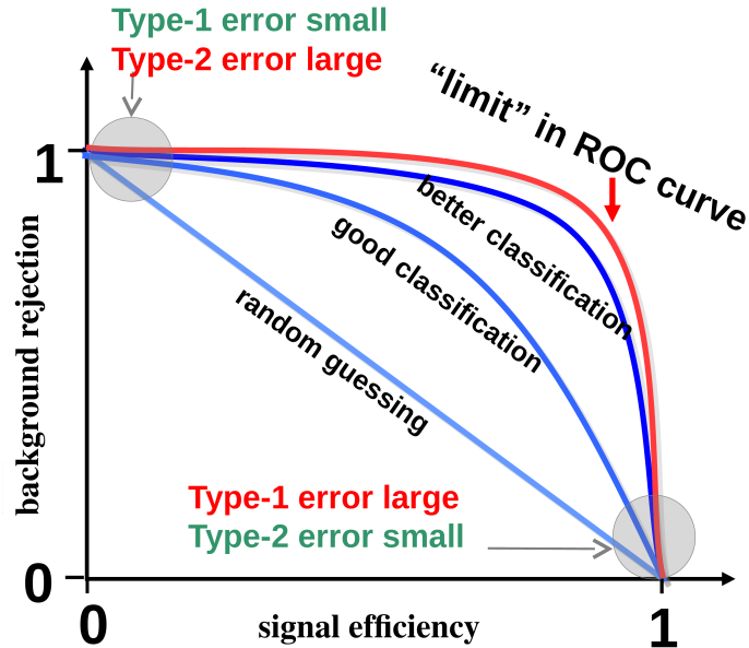
Figure 5.3: The ROC curve, showing the background rejection as a function of the signal efficiency achieved by varying the cut on the MVA output variable y .
