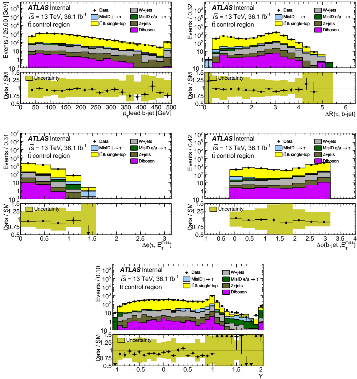
Figure 4.4: Predicted and measured j distribution for the electroweak, top and multi-jet backgrounds in the t\bar{t} enriched control region. Shown are (top left) the p_T of the hardest b -jet, (top right) the \Delta R between the \tau_{\text{had-vis}} candidate and the hardest b -jet, (middle left) the difference in azimuthal angle between the \tau_{\text{had-vis}} candidate and E_T^{\text{miss}} , (middle right) the difference in azimuthal angle between the hardest b -jet and E_T^{\text{miss}} , (bottom) \tau polarisation variable \Upsilon . When plotting the b -jet transverse momentum, the last bin contains overflow. The j \rightarrow \tau background is estimated using the FF method. The uncertainty band in the ratio plots includes both statistical and systematic uncertainties on the background prediction. From [33].
