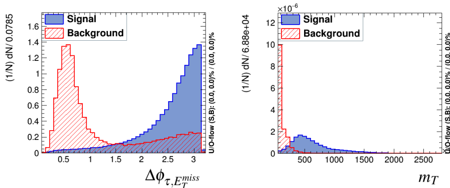
Figure 5.14: Distributions of \Delta\phi_{\tau, E_T^{\text{miss}}} used for default BDT-training and m_T used in place of \Delta\phi_{\tau, E_T^{\text{miss}}} in alternative BDT training for the 500 \leq m_{H^\pm} \leq 2000 GeV mass range. Signal is presented as a blue, solid histogram; top background (as estimated from MC) together with j \rightarrow \tau background (as estimated with FFs) are presented as a red, dashed histogram. Histograms are arbitrarily normalised.
