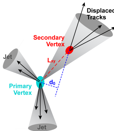
Figure 3.12: Illustration of an event with a b -jet, which shows the b hadron formed from the b quark decays at a secondary vertex at a distance L_{xy} from the primary vertex [77].
