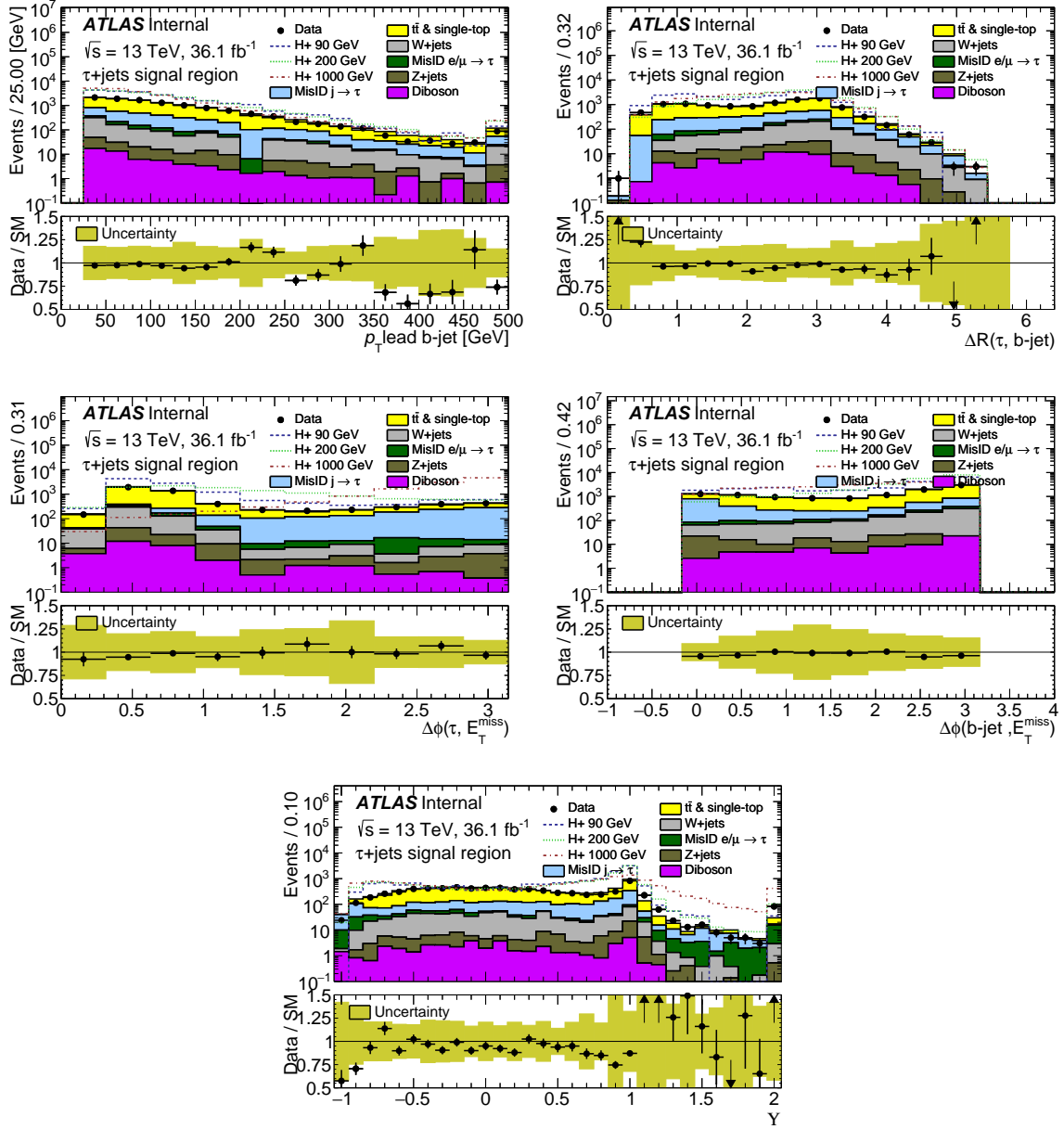
Figure 4.2: Predicted total background distributions along with a few simulated signal samples (with m_{H^\pm} = 90, 200, 1000 GeV), after full event selection. Shown are (top left) the p_T of the hardest b -jet, (top right) the \Delta R between the \tau_{\text{had-vis}} candidate and the hardest b -jet, (middle left) the difference in azimuthal angle between the \tau_{\text{had-vis}} candidate and E_T^{\text{miss}} , (middle right) the difference in azimuthal angle between the hardest b -jet and E_T^{\text{miss}} , (bottom) \tau polarisation variable Y . The background is stacked, while the signal is overlaid. When plotting the b -jet transverse momentum, the last bin contains overflow. The j \rightarrow \tau background is estimated using the FF method. The uncertainty band in the ratio plots includes both statistical and systematic uncertainties on the background prediction. The signal distributions are all scaled to the integral of the total background. From [33].
