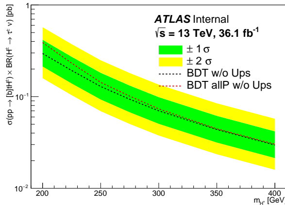
Figure 5.23: Expected 95% CL exclusion limits on \sigma(pp \rightarrow [b]tH^\pm) \times \text{BR}(H^\pm \rightarrow \tau^\pm \nu) for charged Higgs boson production as a function of m_{H^\pm} in 36.1 \text{ fb}^{-1} of pp collision data at \sqrt{s} = 13 \text{ TeV} for comparison of BDT output when the BDT training is performed separately for events with a selected 1- or 3-prong \tau_{\text{had-vis}} object. This study is done for H^\pm masses in the range 200 – 400 GeV with the p_T^{\tau\text{-track}} in place of \Upsilon included in the final BDT discriminant (BDT w/o Ups), with the BDT output when the BDT training is performed for all events together (BDT allP w/o Ups).
