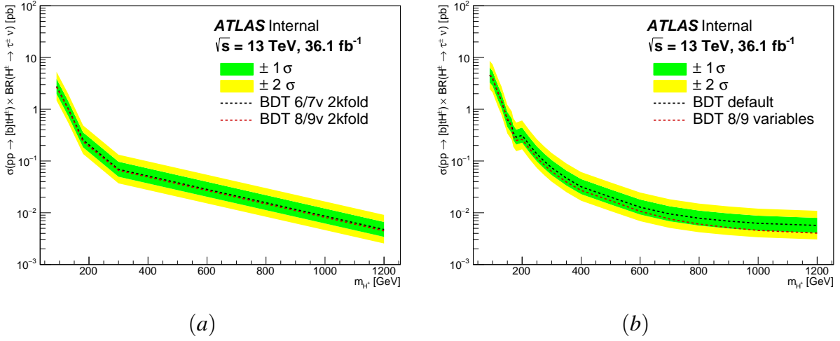
Figure 5.18: Juxtaposition of expected 95% CL exclusion limits on \sigma(pp \rightarrow [b]tH^\pm) \times \text{BR}(H^\pm \rightarrow \tau^\pm \nu) for charged Higgs boson production as a function of m_{H^\pm} in 36.1 \text{ fb}^{-1} of pp collision data at \sqrt{s} = 13 \text{ TeV} for two cases: (a) BDT output built by set of 6/7 input variables and BDT built by set of 8/9 input variables, with k\text{-fold}=2 training method. Here, only 5 mass points: 90, 130, 180, 300 and 1200 GeV are used for the limits study; (b) default BDT output and an alternative BDT built by set of 8/9 input variables with k\text{fold}=5 used, and all available mass points used for the limits study.
