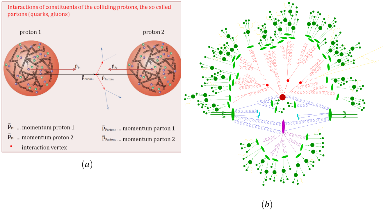
Figure A.1: (a) schematic overview of a pp collision. (b) sketch of a hadron-hadron collision as simulated by a Monte-Carlo event generator. The red blob in the center represents the hard collision, surrounded by a tree-like structure representing Bremsstrahlung as simulated by parton showers. The purple blob indicates a secondary hard scattering event. Parton-to-hadron transitions are represented by light green blobs, dark green blobs indicate hadron decays, while yellow lines signal soft photon radiation. From [59, 151].
