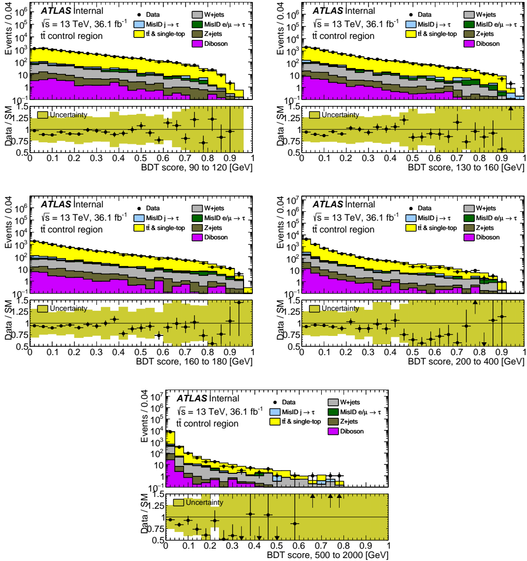
Figure 5.11: Predicted and measured BDT score distributions in the t\bar{t} enriched control region. Shown are five H^\pm mass range trainings. The j \rightarrow \tau background is estimated using the FF method. The uncertainty bands in the ratio plots include both the statistical and systematic uncertainties of simulated events, added in quadrature. From [33].
