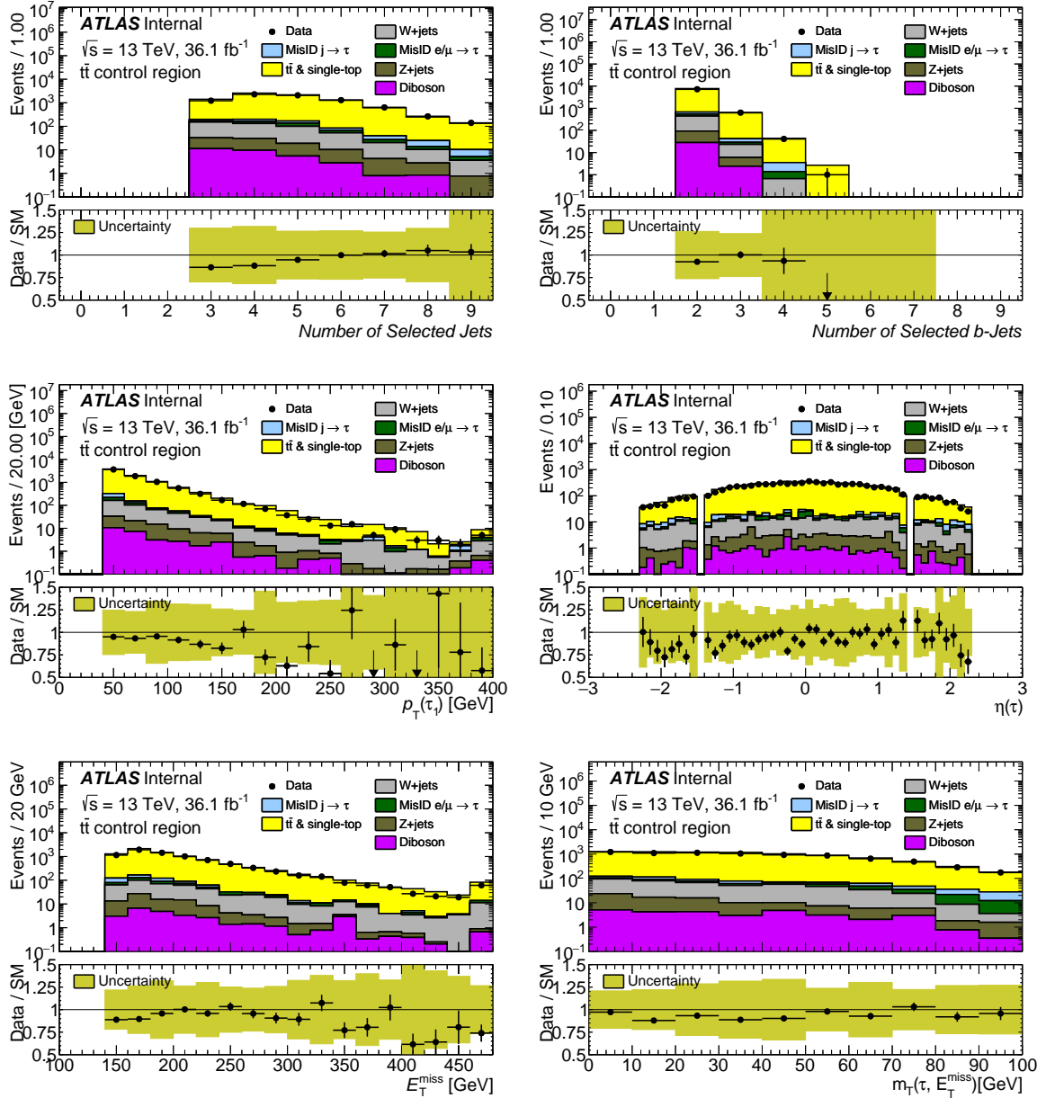
Figure 4.3: Predicted and measured distribution for the electroweak, top and multi-jet backgrounds in the t\bar{t} enriched control region. Shown are (top left) the number of reconstructed jets, (top right) the number of b -tagged jets, (middle left) the \tau_{\text{had-vis}} candidate p_T , (middle right) the \tau_{\text{had-vis}} candidate \eta , (bottom left) E_T^{\text{miss}} and (bottom right) the transverse mass of the \tau_{\text{had-vis}} candidate and E_T^{\text{miss}} . When plotting the transverse momenta and mass, the last bin contains overflow. The j \rightarrow \tau background is estimated using the FF method. The uncertainty band in the ratio plots includes both statistical and systematic uncertainties on the background prediction. From [33].
