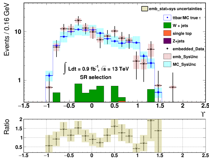
Figure 6.19: \Upsilon distributions in logarithmic scale of the \mu \rightarrow \tau embedded 2015 data sample of events with a true 1-prong \tau_{\text{had-vis}} compared to default simulation after applying the SR selection.
