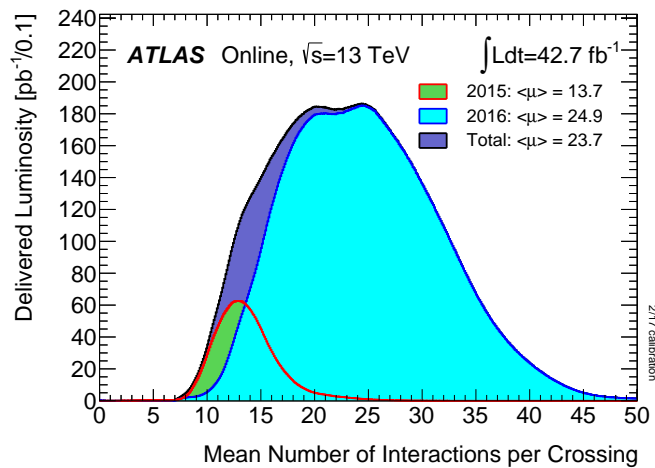
Figure 3.7: Distribution of the mean number of interactions per bunch crossing, i.e. pile-up weighted by luminosity for data taken in 2015 and 2016 [54].
