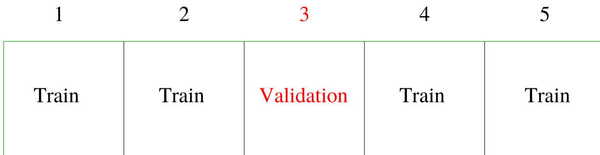
Figure 5.6: For the k -th part (third above), the model is fitting to the other K - 1 parts of the data, and calculation of the prediction error of the fitted model during predicting the k -th part of the data is done. The procedure is repeated for k = 1, 2, \dots, K and combination of the K estimates of prediction error is prepared [126].
