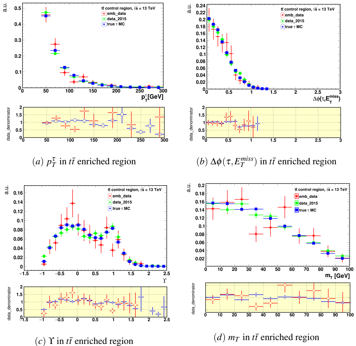
Figure 6.17: Juxtaposition between 2015 data, embedding data and true \tau leptons from MC simulations of following distributions: (a) p_T^\tau , (b) \Delta\phi(\tau, E_T^{miss}) , (c) \Upsilon and (d) m_T , in t\bar{t} enriched CR where 2015 data are always on denominator in ratio plots. Only statistical uncertainties are shown.
