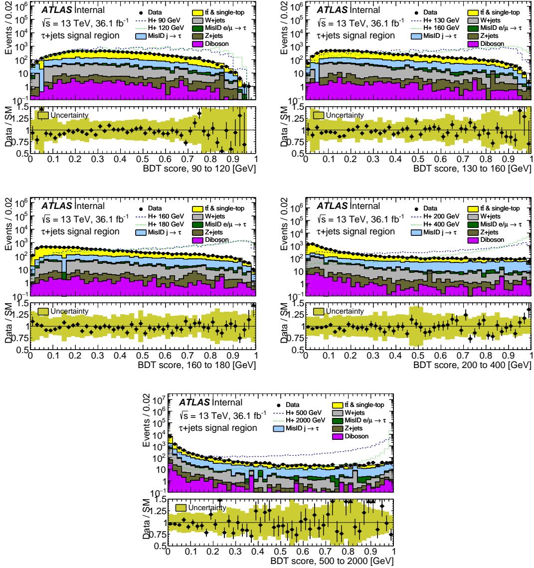
Figure 5.12: BDT score distributions in signal region. Shown are five H^\pm mass range trainings. The j \rightarrow \tau background is estimated using the FF method. The uncertainty bands in the ratio plots include both the statistical and systematic uncertainties of simulated events, added in quadrature. The normalisation of the signal samples corresponds to the integral of the background. From [33].
