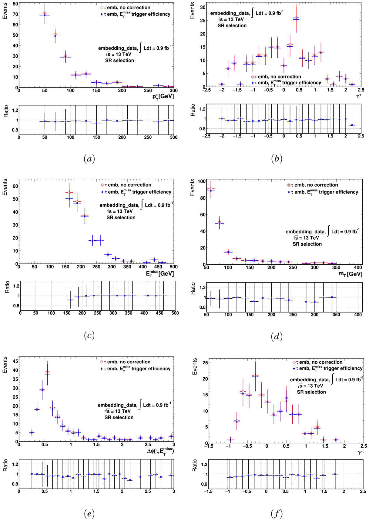
Figure 6.10: Juxtaposition of (a) p_T^\tau , (b) \eta^\tau , (c) E_T^{miss} , (d) m_T , (e) \Delta\phi(\tau, E_T^{miss}) and (f) Y^\tau observables before and after applying the correction on E_T^{miss} trigger efficiency for data embedding.
