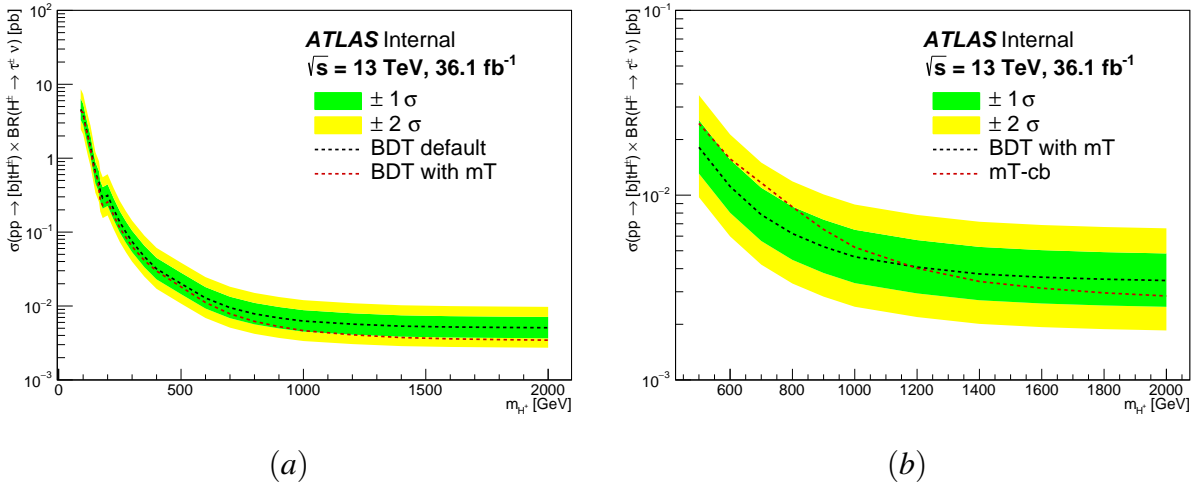
Figure 5.13: Expected 95% CL exclusion limits on \sigma(pp \rightarrow [b]tH^\pm) \times \text{BR}(H^\pm \rightarrow \tau^\pm \nu) for charged Higgs boson production as a function of m_{H^\pm} in 36.1 \text{ fb}^{-1} of pp collision data at \sqrt{s} = 13 TeV for (a) default BDT output and alternative BDT output where m_T in place of \Delta\phi_{\tau, E_T^{\text{miss}}} is used as an input variable; (b) BDT output, where m_T in place of \Delta\phi_{\tau, E_T^{\text{miss}}} is used as an input variable and cut based analysis limit based on m_T variable, m_T -cb.
