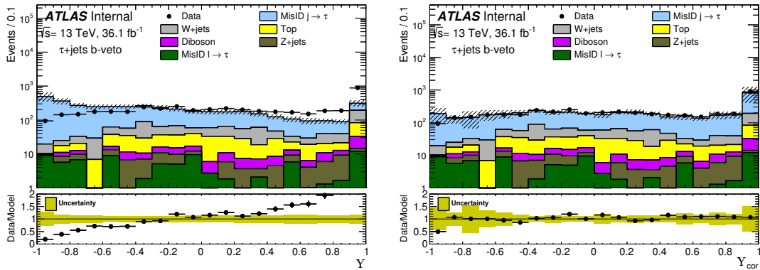
Figure 4.8: Distribution of Y variable before (left) and after (right) Smirnov transformation in the signal-like region with a b -jet veto applied. From [33].
