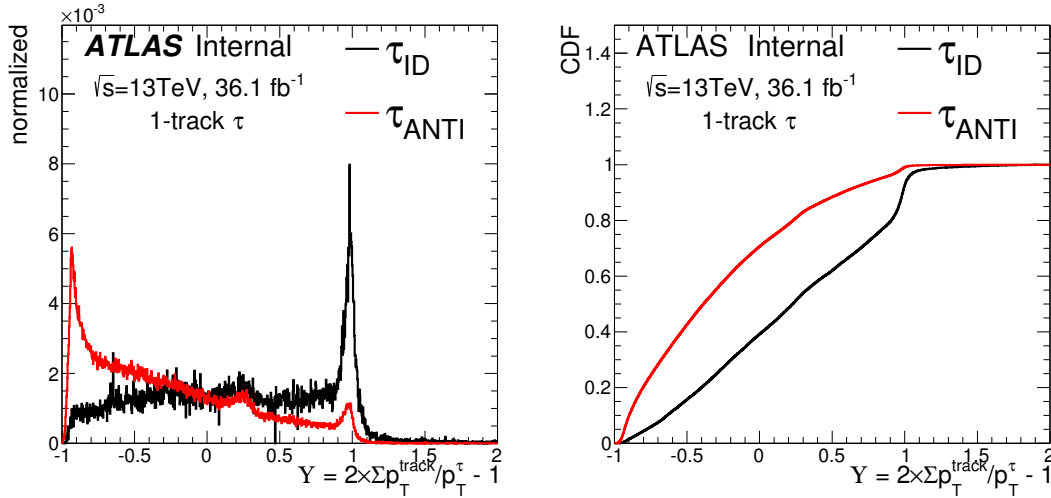
Figure 4.7: Left: Distribution of the \Upsilon variable for \tau_{\text{had-vis}} (black) and anti- \tau_{\text{had-vis}} (red) candidates in the W +jets CR. Right: F(\Upsilon) of \Upsilon for \tau_{\text{had-vis}} (black) and anti- \tau_{\text{had-vis}} (red) candidates in the W +jets CR. From [33].
