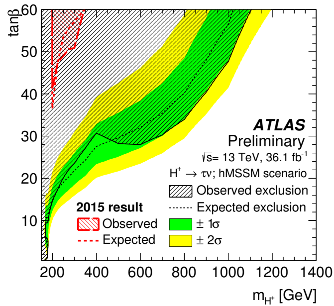
Figure 7.4: 95% CL exclusion limits on \tan\beta as a function of m_{H^\pm} , shown in the context of the hMSSM, for the regions in which theoretical predictions are available ( 0.5 \leq \tan\beta \leq 60 ). In the case of the expected limits, one- and two-standard-deviation uncertainty bands are also shown. As a comparison, the red curves show the observed and expected exclusion limits based on the dataset of 3.2\text{ fb}^{-1} collected in 2015 at \sqrt{s} = 13\text{ TeV} . From [12].
