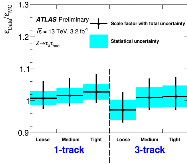
Figure 6.11: The scale factors ( \epsilon_{\text{Data}}/\epsilon_{\text{MC}} ) needed to bring the \tau identification efficiency in simulation ( \epsilon_{\text{MC}} ) to the level observed in data ( \epsilon_{\text{Data}} ) for one and three tracks (prongs) \tau_{\text{had-vis}} candidates with p_T > 20 GeV. The combined systematic and statistical uncertainties are shown. From [142].
