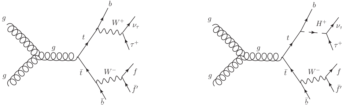
Figure 6.1: Feynman diagrams for the dominant process giving the SM background, top quark pair production, (left) and the charged Higgs boson signal production for m_{H^\pm} < m_{top} (right).
