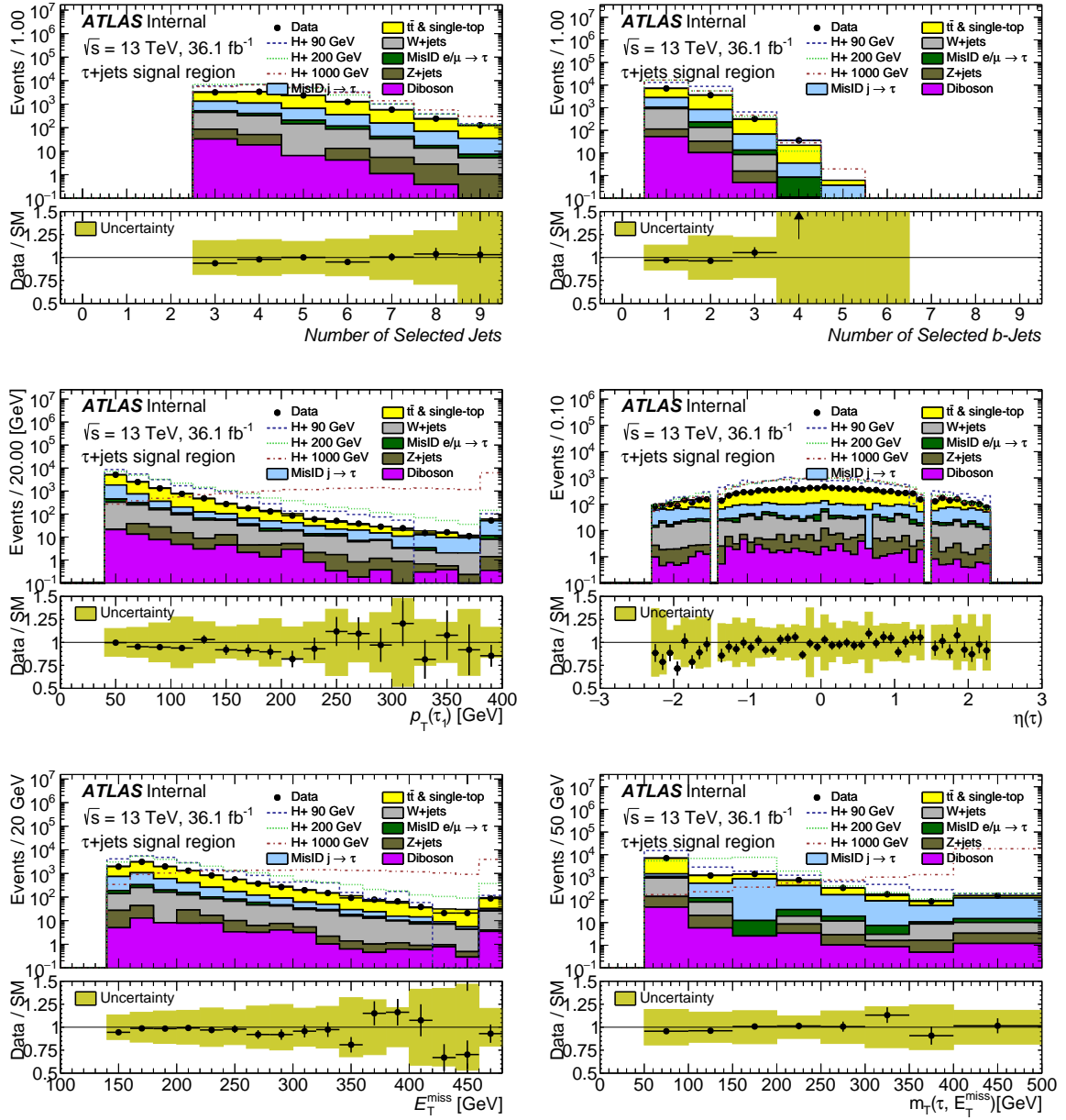
Figure 4.1: Predicted total background distributions along with a few simulated signal samples (with m_{H^\pm} = 90, 200, 1000 GeV), after full event selection. Shown are (top left) the number of reconstructed jets, (top right) the number of b -tagged jets, (middle left) the \tau_{\text{had-vis}} candidate p_T , (middle right) the \tau_{\text{had-vis}} candidate \eta , (bottom left) E_T^{\text{miss}} and (bottom right) the transverse mass of the \tau_{\text{had-vis}} candidate and E_T^{\text{miss}} . The background is stacked, while the signal is overlaid. When plotting the transverse momenta and mass, the last bin contains overflow. The j \rightarrow \tau background is estimated using the FF method. The uncertainty band in the ratio plots includes both statistical and systematic uncertainties on the background prediction. The signal distributions are all scaled to the integral of the total background. From [33].
